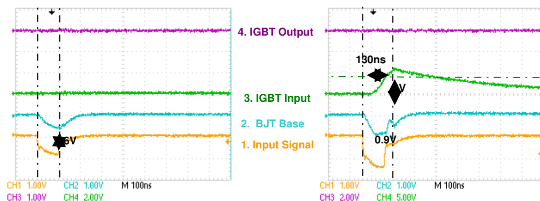
Fig 4.5 System response at low ( <1.2\text{V} ) pulsing amplitude
