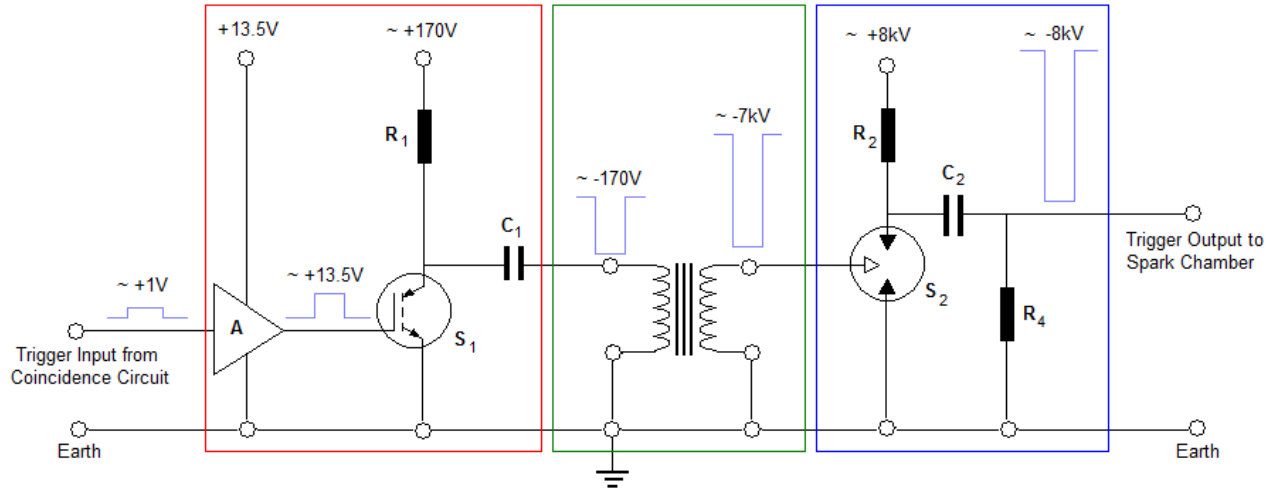
Fig 3.2 Simplified circuit diagram illustrating the primary components of the NIKHEF pulsing circuit. There are three distinct phases of amplification – a ‘low’ voltage circuit switches the IGBT, S_1 ; a step-up transformer; a triggered spark gap, S_2 . Note that both IGBT and spark gap are driven as described in section 3.1. Stages of amplification are indicated by the evolution of a \sim 1\text{V} square wave to an 8\text{kV} output pulse.
