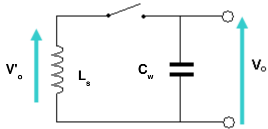
Fig 5.7 Simplest equivalent circuit for the transformer output.
