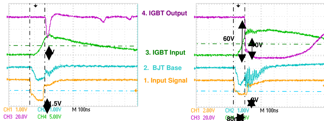
Fig 4.6 System response at high ( >1.2V ) pulsing amplitude
