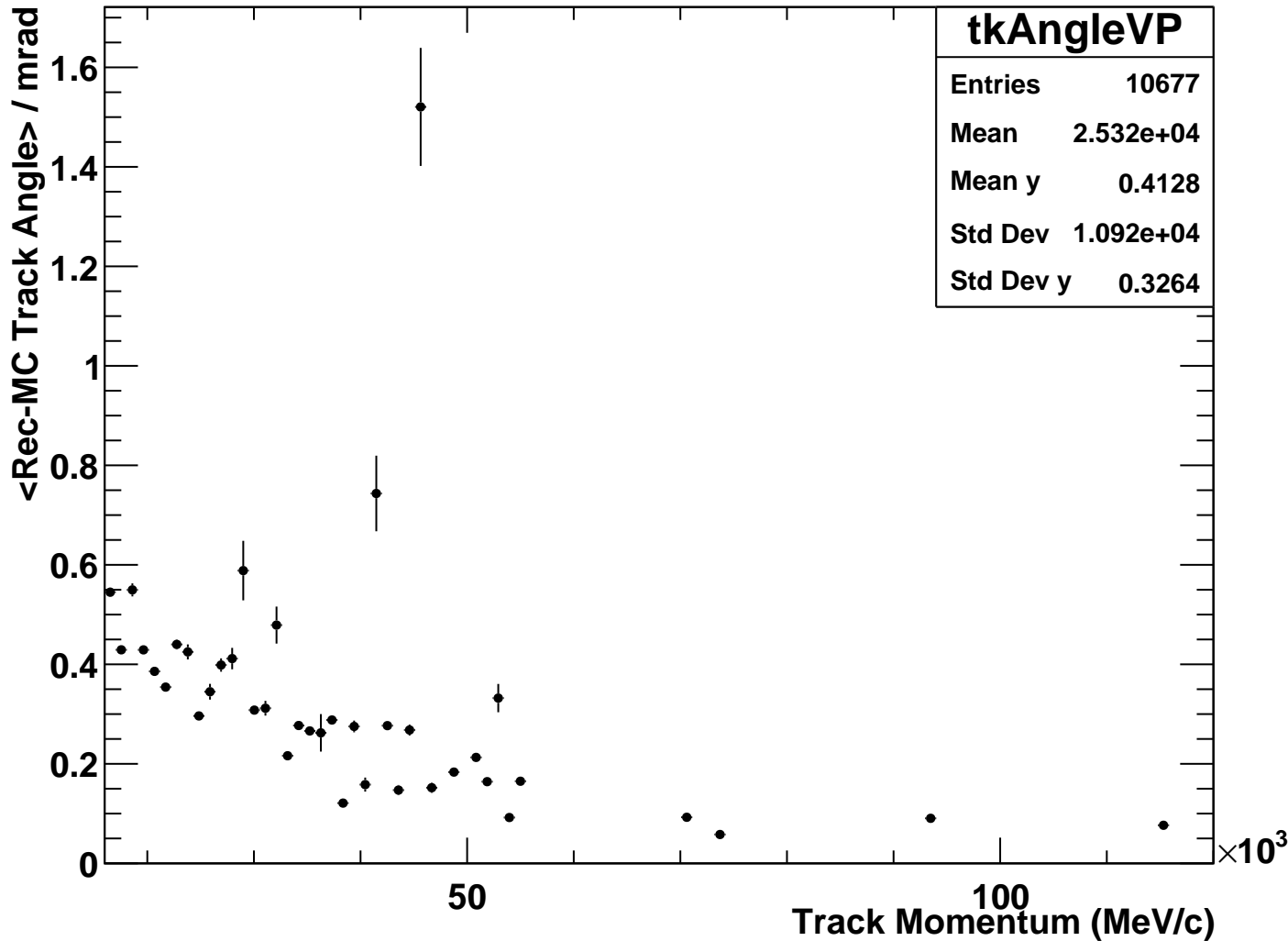
Rich2Gas <Angle between TkNeg Reco and MC Track Direction> Versus Momentum
