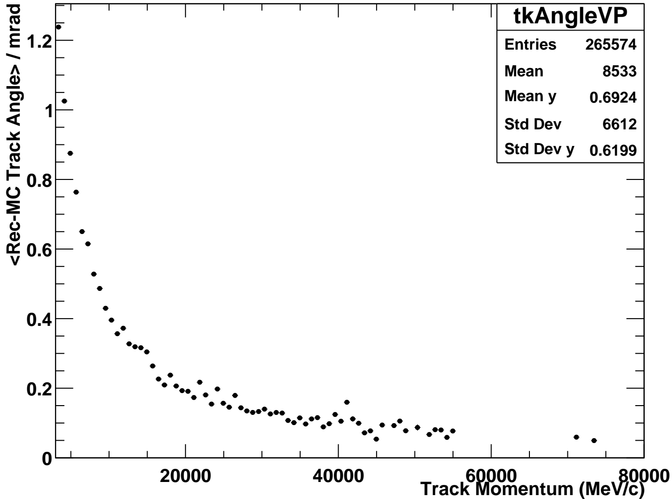
Rich1Gas <Angle between TkNeg Reco and MC Track Direction> Versus Momentum
