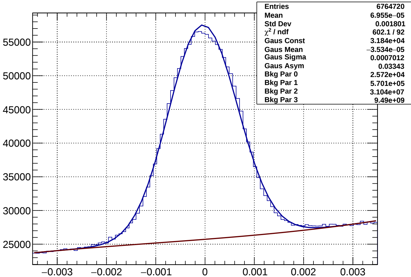
Rich2Gas muon Rec-Exp CKtheta - Bin 23 Ptot 27.985 to 29.18 GeV
