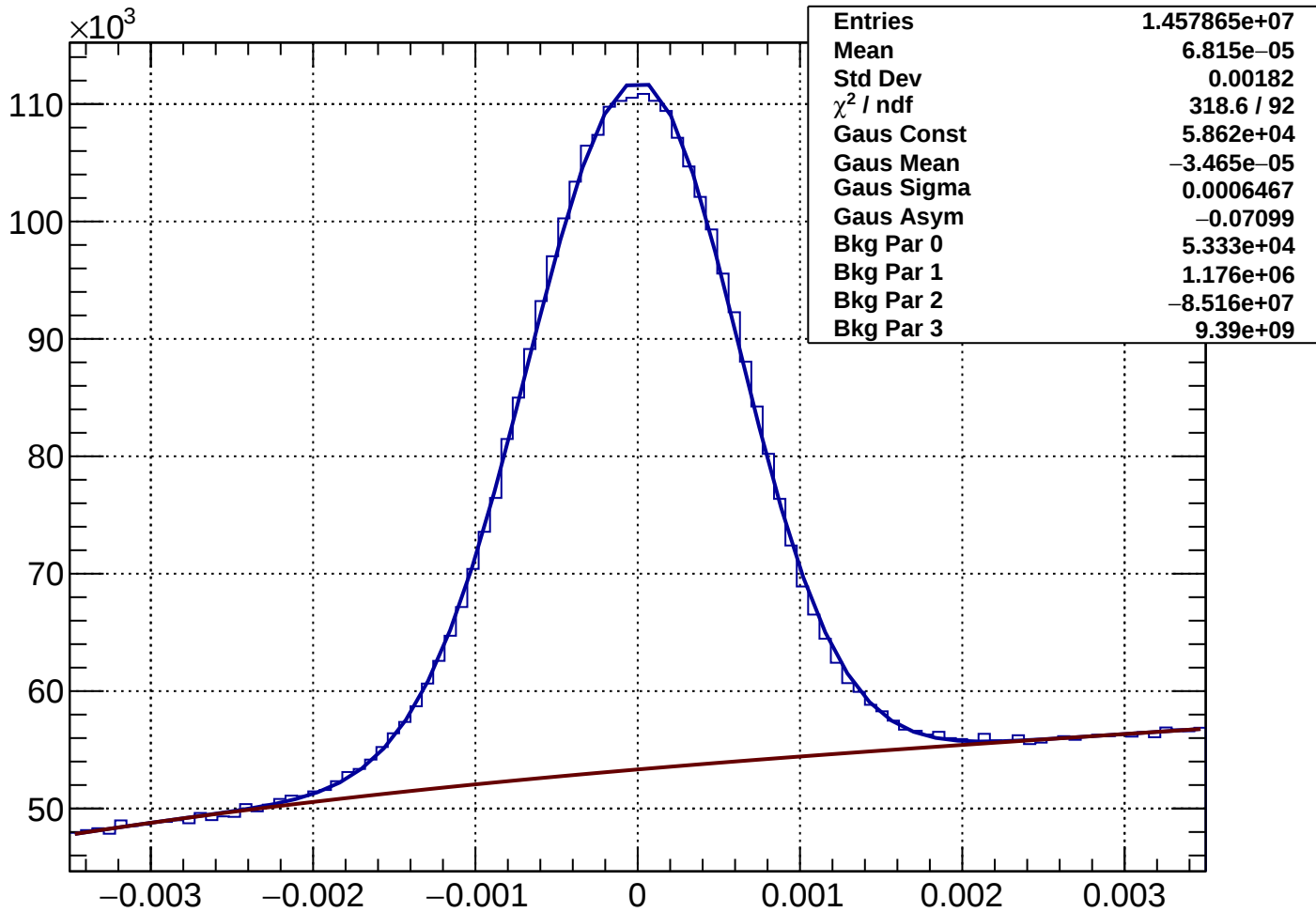
Rich2Gas muon Rec-Exp CKtheta - Bin 20 Ptot 24.4 to 25.595 GeV
