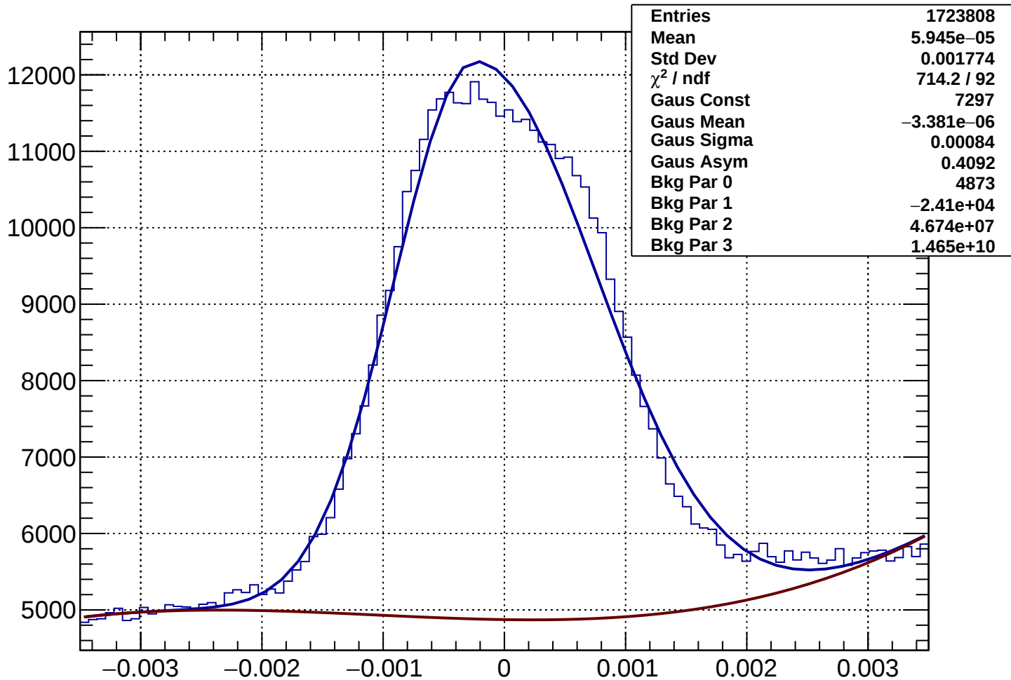
Rich2Gas muon Rec-Exp CKtheta - Bin 31 Ptot 37.545 to 38.74 GeV
