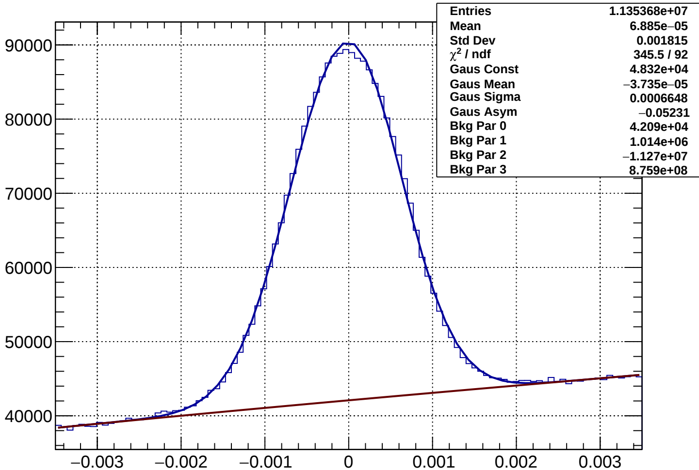
Rich2Gas muon Rec-Exp CKtheta - Bin 21 Ptot 25.595 to 26.79 GeV
