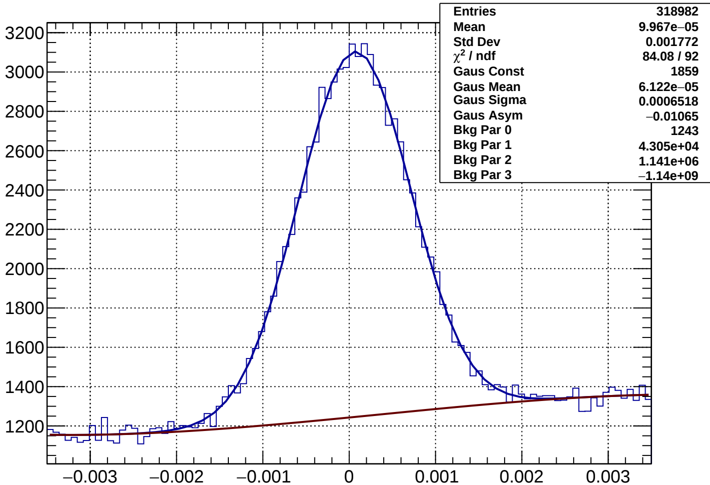
Rich2Gas muon Rec-Exp CKtheta - Bin 91 Ptot 109.245 to 110.44 GeV
