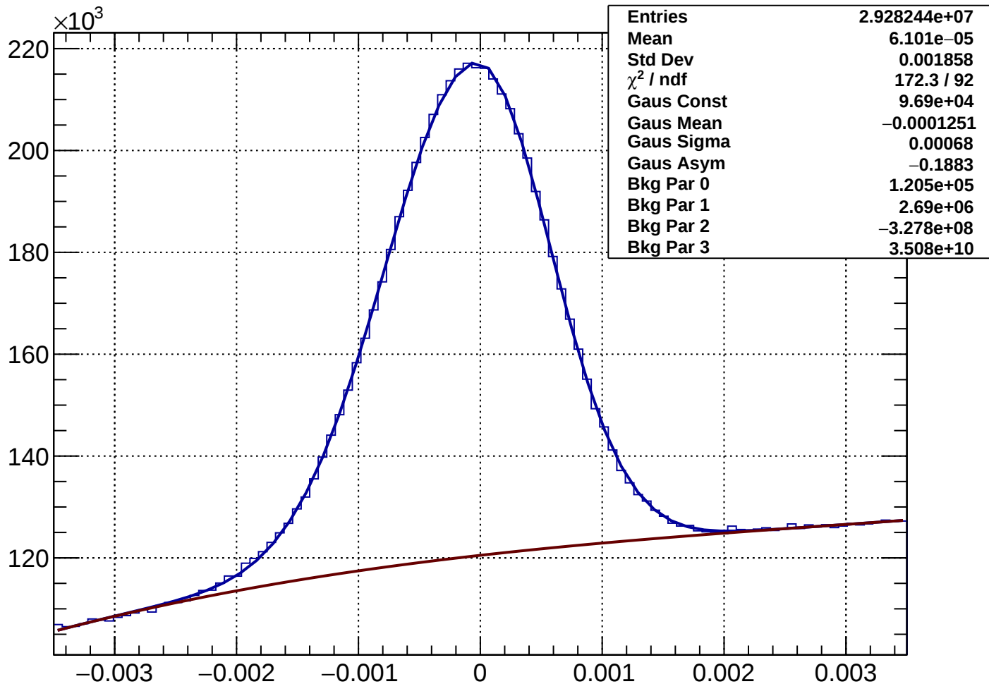
Rich2Gas muon Rec-Exp CKtheta - Bin 13 Ptot 16.035 to 17.23 GeV
