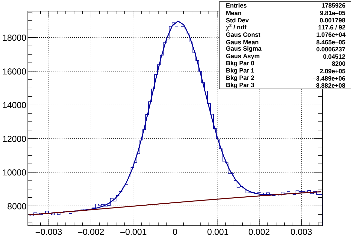
Rich2Gas muon Rec-Exp CKtheta - Bin 99 Ptot 118.805 to 120 GeV
