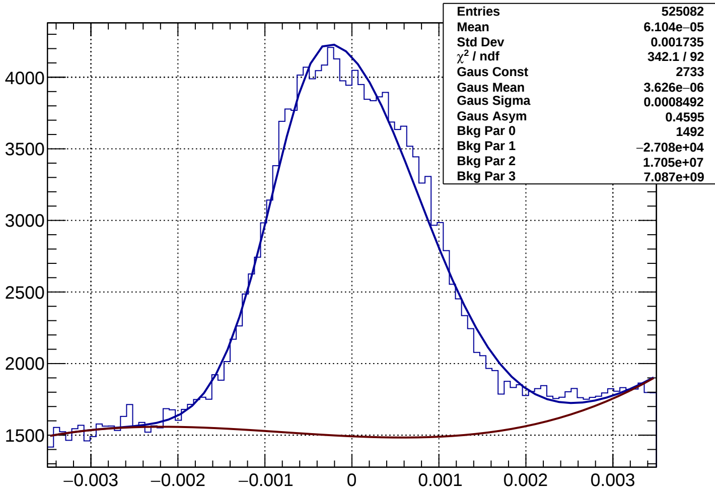
Rich2Gas muon Rec-Exp CKtheta - Bin 33 Ptot 39.935 to 41.13 GeV
