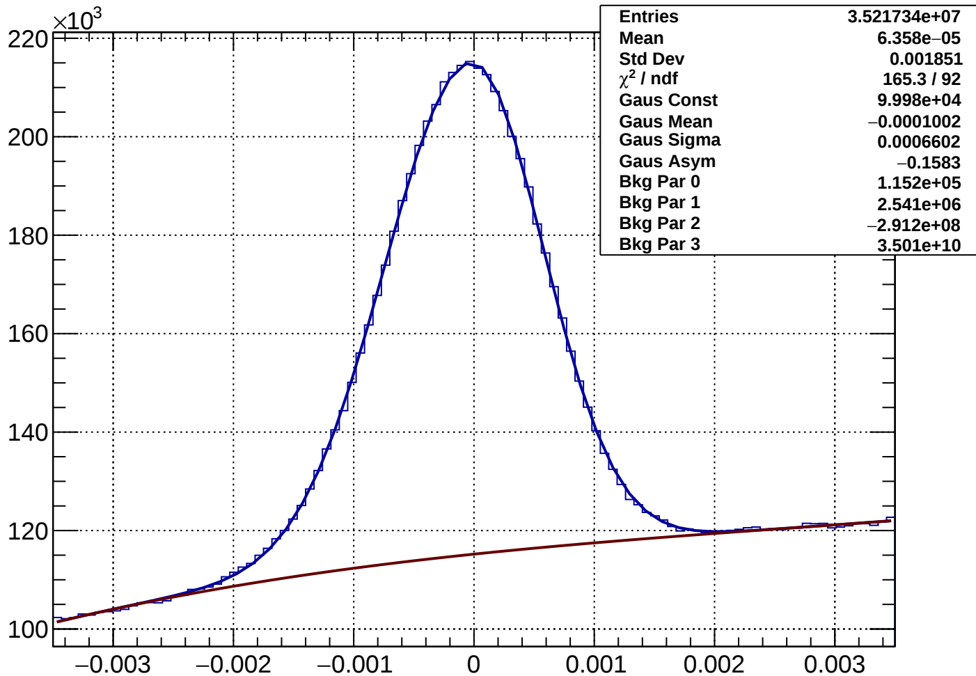
Rich2Gas muon Rec-Exp CKtheta - Bin 14 Ptot 17.23 to 18.425 GeV
