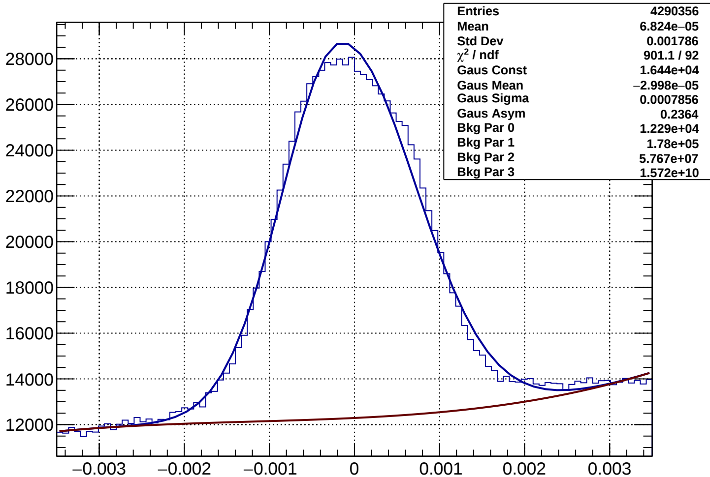
Rich2Gas muon Rec-Exp CKtheta - Bin 27 Ptot 32.765 to 33.96 GeV
