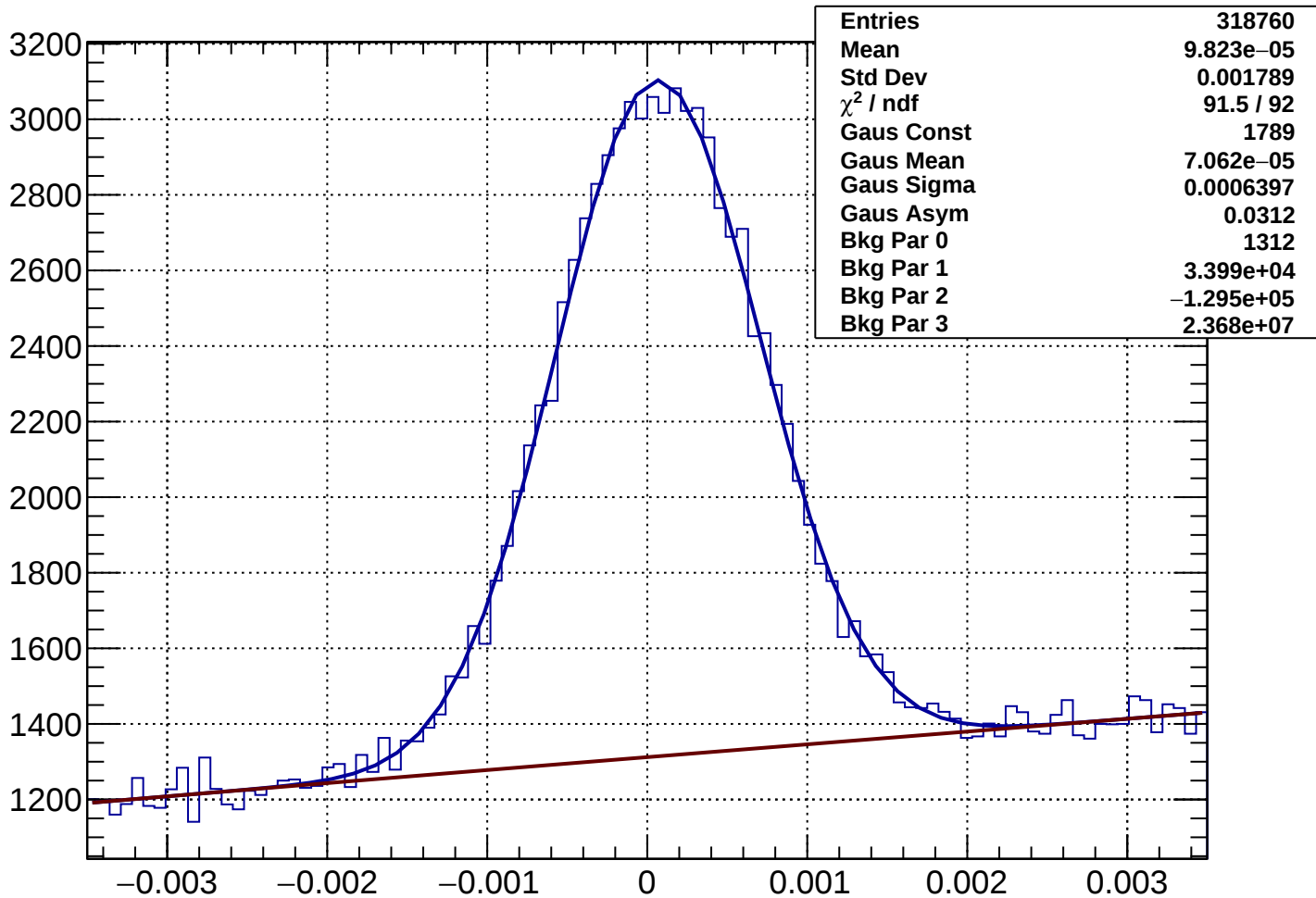
Rich2Gas muon Rec-Exp CKtheta - Bin 98 Ptot 117.61 to 118.805 GeV
