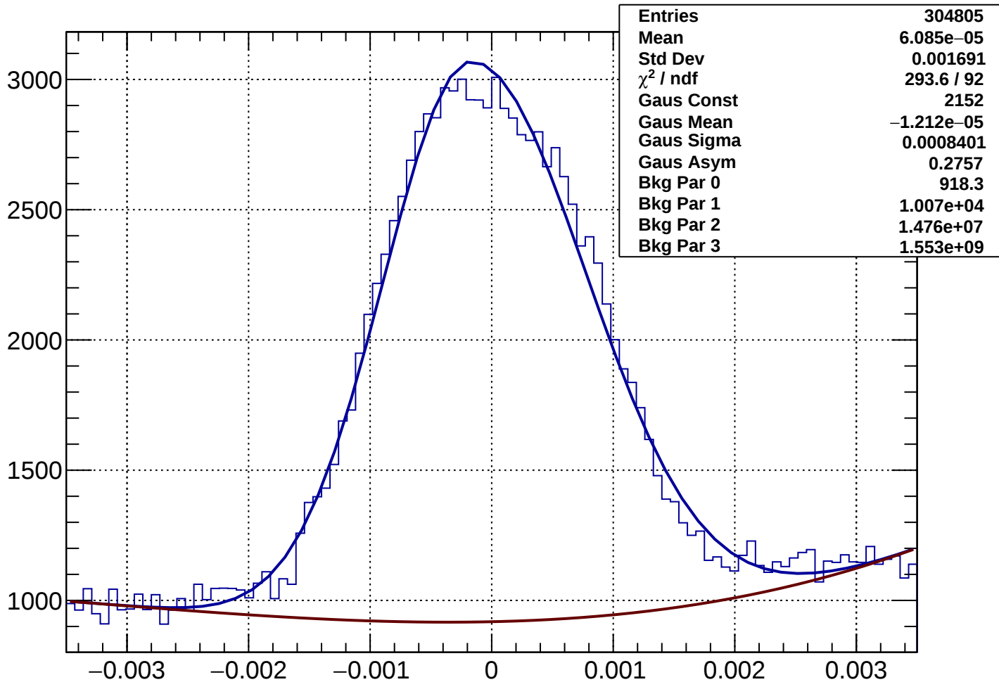
Rich2Gas muon Rec-Exp CKtheta - Bin 82 Ptot 98.49 to 99.685 GeV
