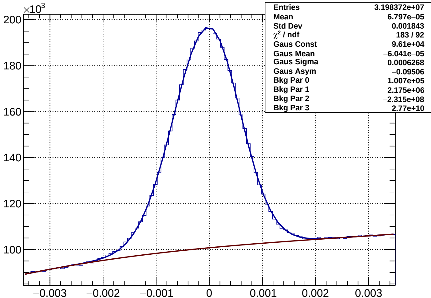
Rich2Gas muon Rec-Exp CKtheta - Bin 16 Ptot 19.62 to 20.815 GeV
