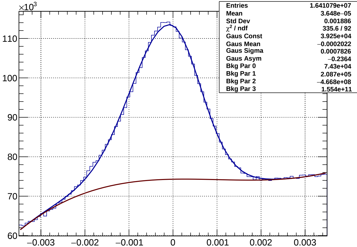
Rich2Gas muon Rec-Exp CKtheta - Bin 9 Ptot 11.255 to 12.45 GeV
