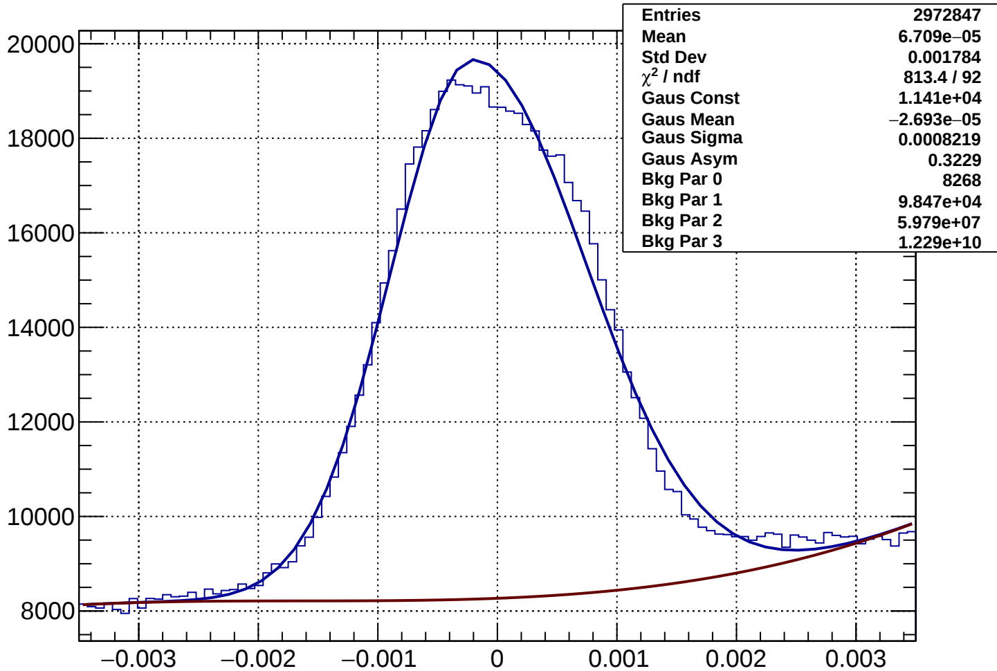
Rich2Gas muon Rec-Exp CKtheta - Bin 29 Ptot 35.155 to 36.35 GeV
