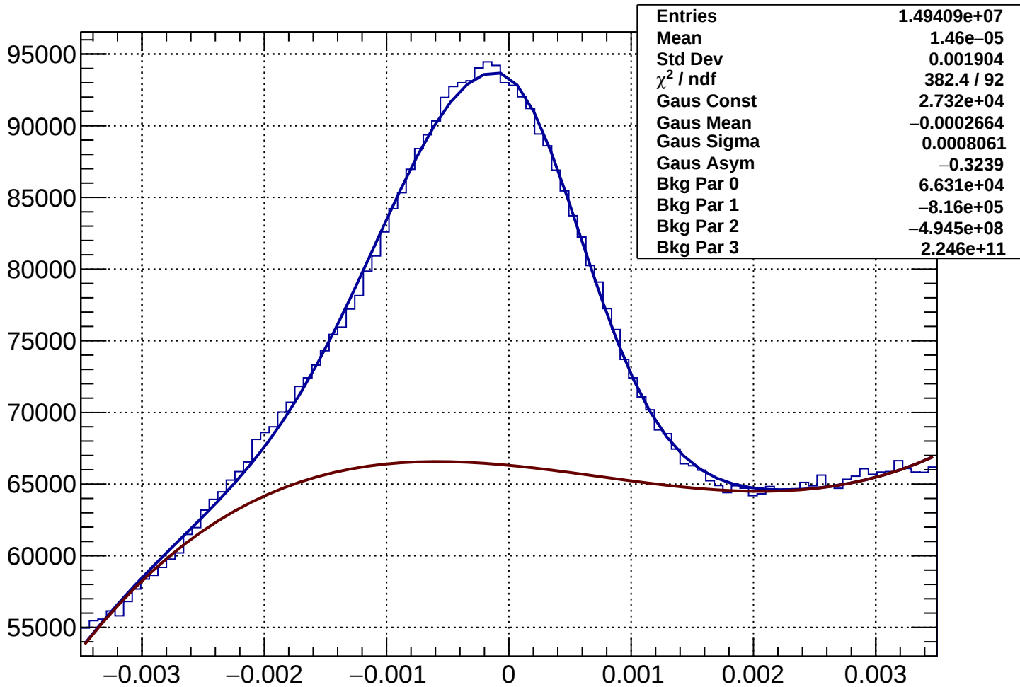
Rich2Gas muon Rec-Exp CKtheta - Bin 8 Ptot 10.06 to 11.255 GeV
