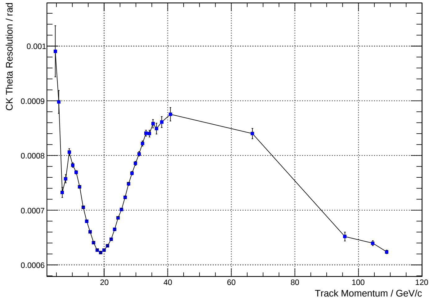
Rich2Gas Both muon CK Theta Resolution Versus Momentum
