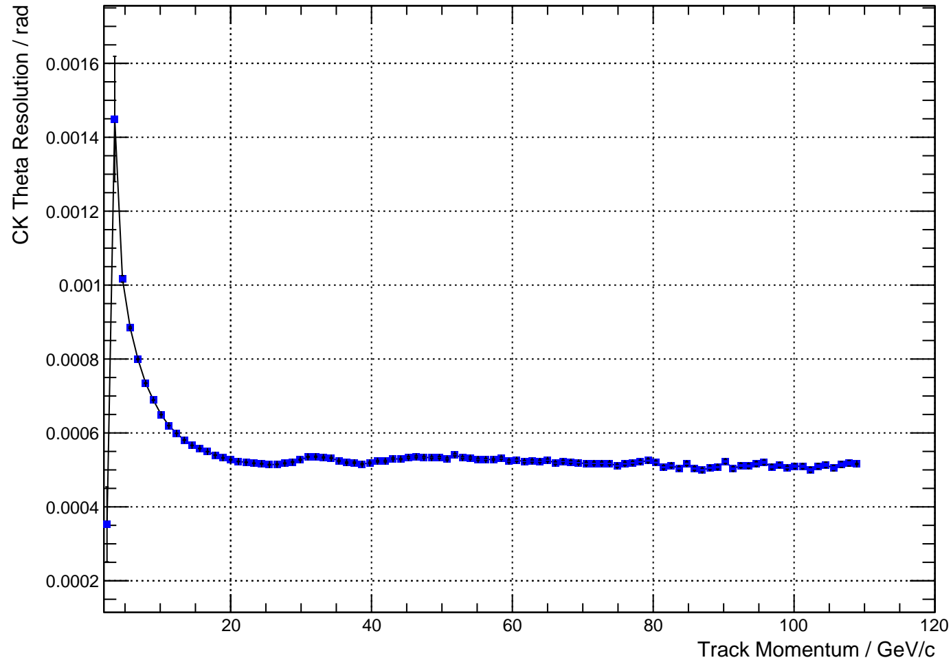
Rich2Gas Both All CK Theta Resolution Versus Momentum
