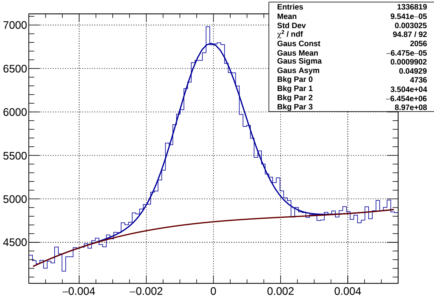
Rich1Gas proton Rec-Exp CKtheta - Bin 50 Ptot 60.25 to 61.445 GeV
