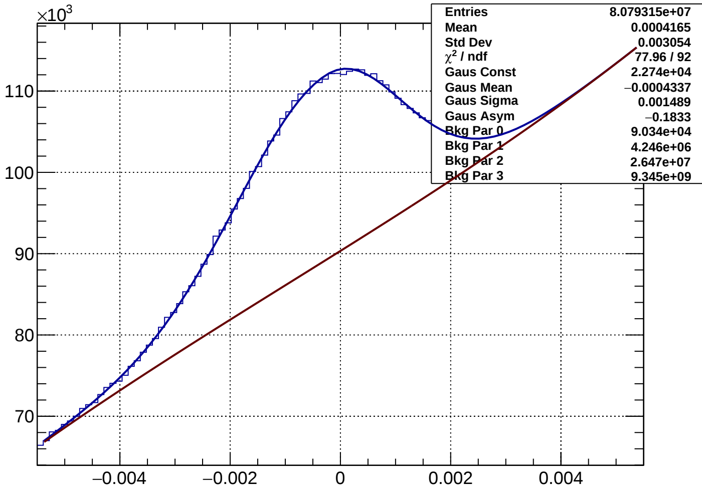
Rich1Gas proton Rec-Exp CKtheta - Bin 15 Ptot 18.425 to 19.62 GeV
