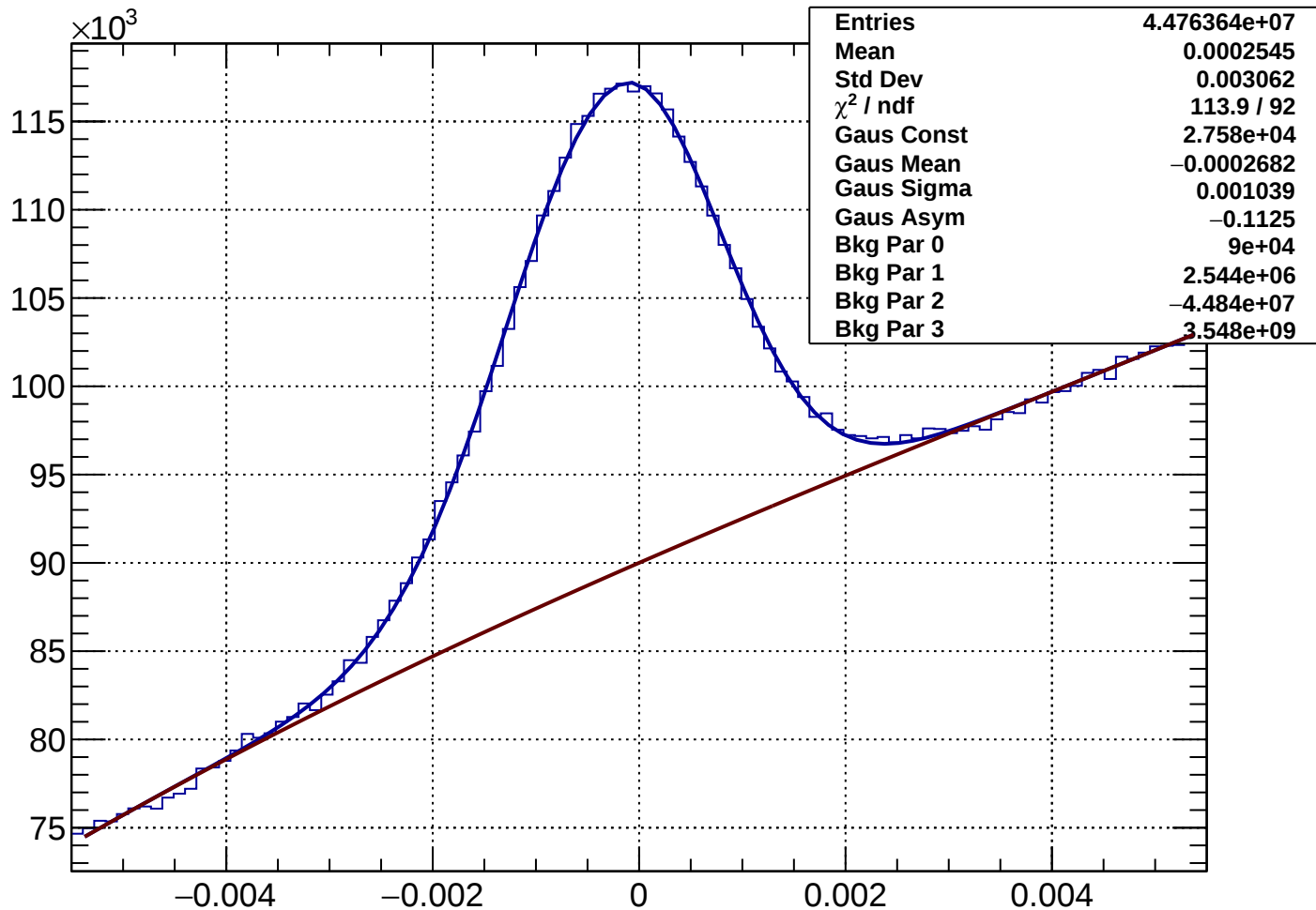
Rich1Gas proton Rec-Exp CKtheta - Bin 18 Ptot 22.01 to 23.205 GeV
