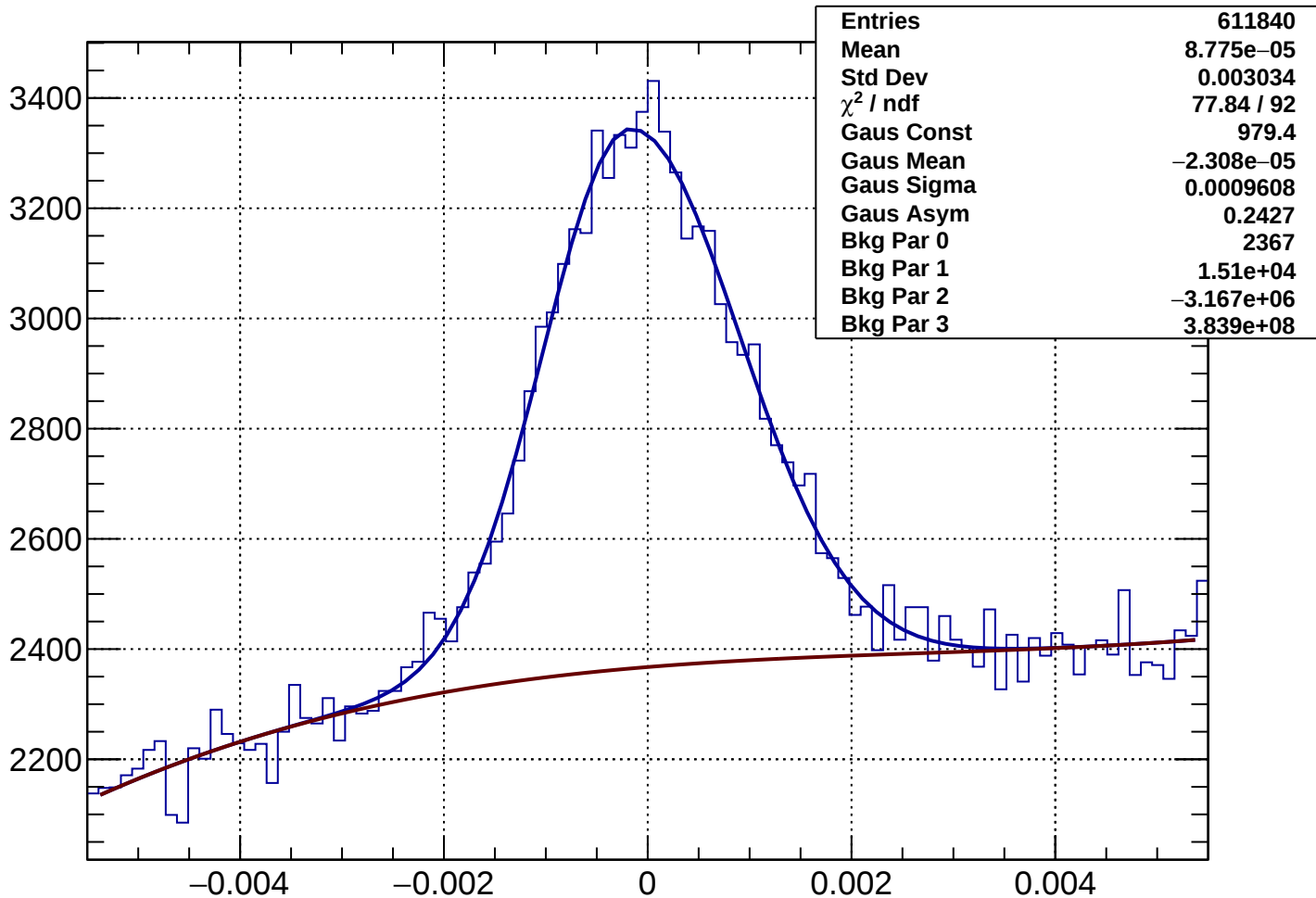
Rich1Gas proton Rec-Exp CKtheta - Bin 60 Ptot 72.2 to 73.395 GeV
