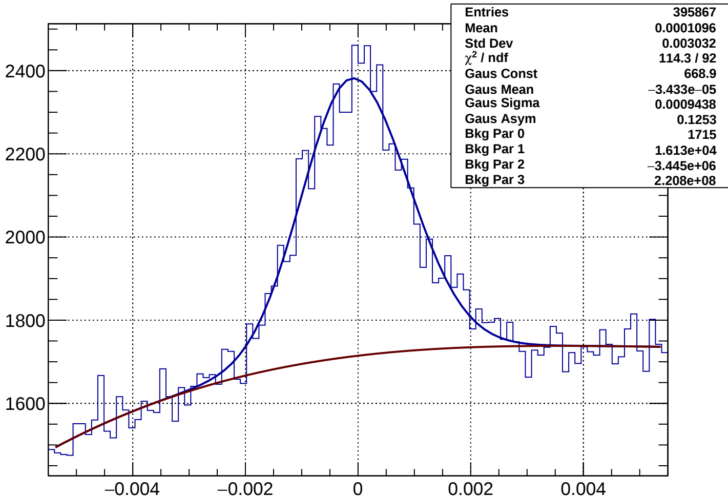
Rich1Gas proton Rec-Exp CKtheta - Bin 87 Ptot 104.465 to 105.66 GeV
