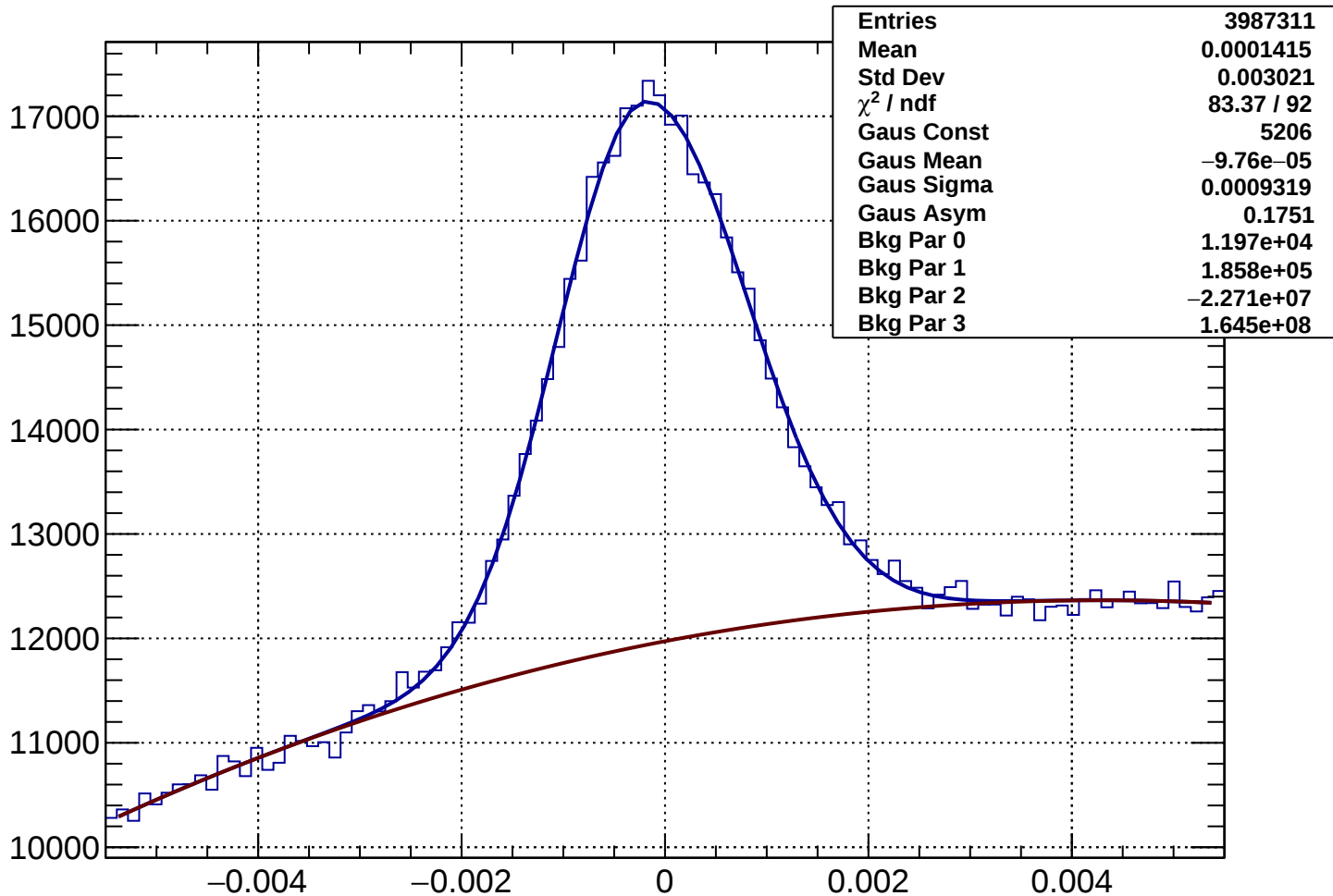
Rich1Gas proton Rec-Exp CKtheta - Bin 37 Ptot 44.715 to 45.91 GeV
