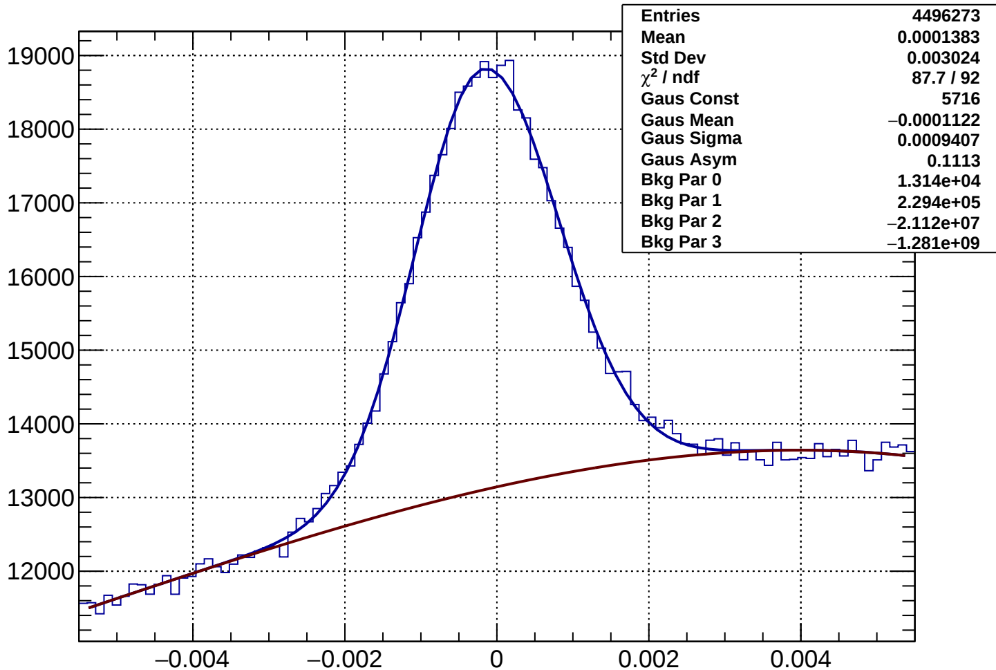
Rich1Gas proton Rec-Exp CKtheta - Bin 36 Ptot 43.52 to 44.715 GeV
