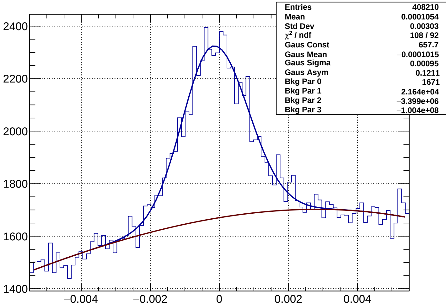
Rich1Gas proton Rec-Exp CKtheta - Bin 67 Ptot 80.565 to 81.76 GeV
