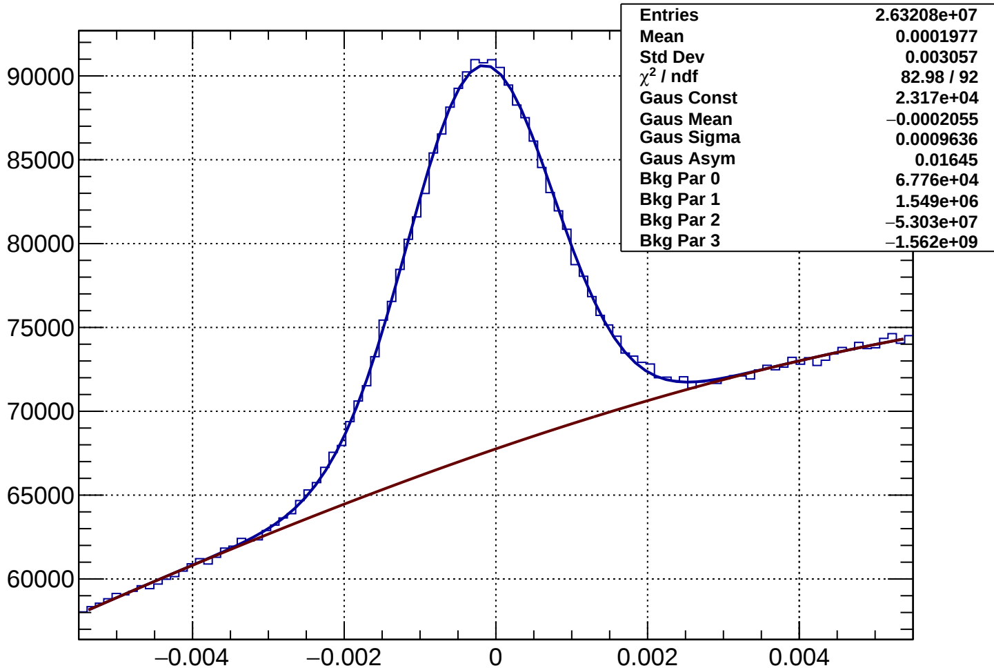
Rich1Gas proton Rec-Exp CKtheta - Bin 21 Ptot 25.595 to 26.79 GeV
