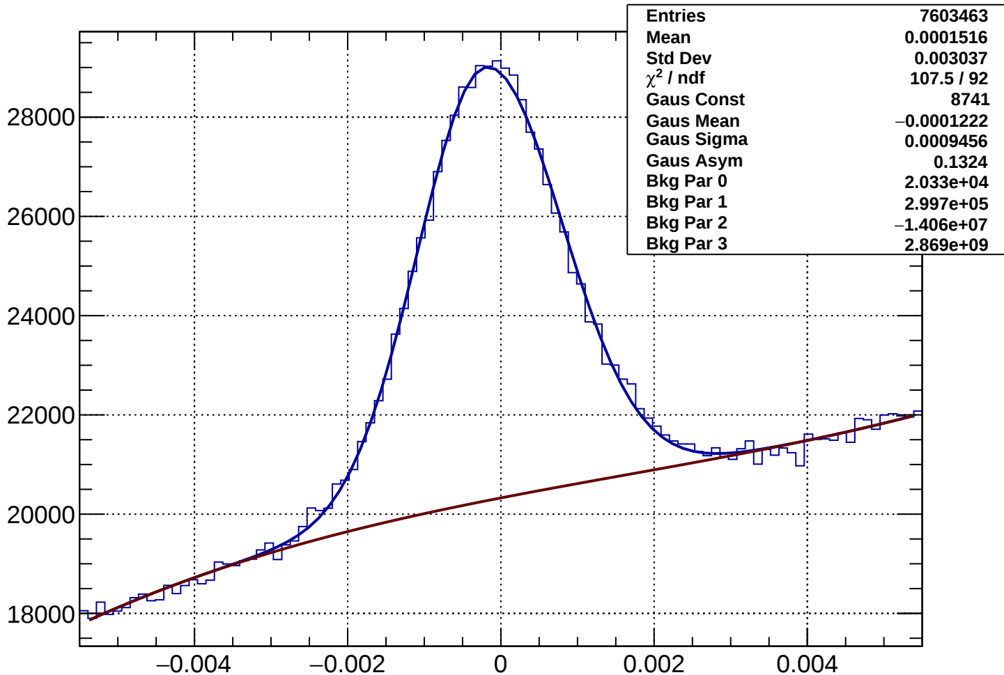
Rich1Gas proton Rec-Exp CKtheta - Bin 31 Ptot 37.545 to 38.74 GeV
