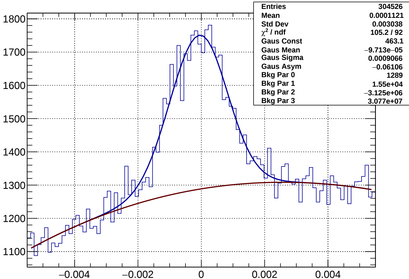
Rich1Gas proton Rec-Exp CKtheta - Bin 72 Ptot 86.54 to 87.735 GeV
