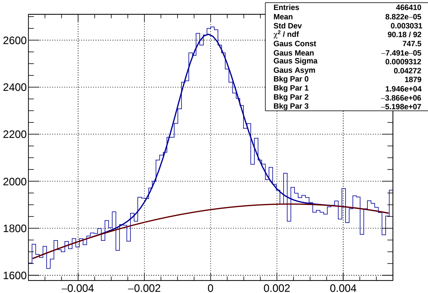
Rich1Gas proton Rec-Exp CKtheta - Bin 64 Ptot 76.98 to 78.175 GeV
