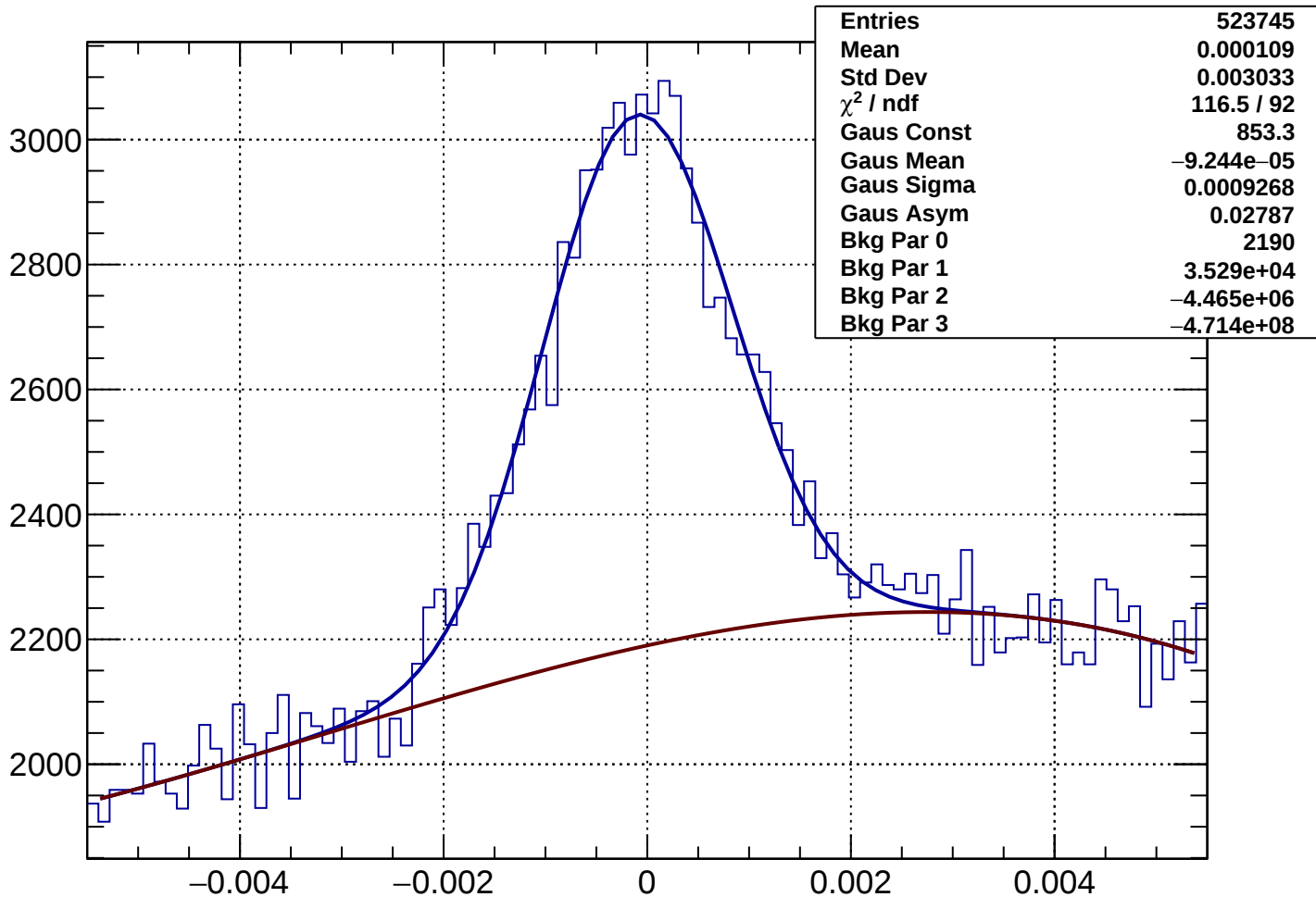
Rich1Gas proton Rec-Exp CKtheta - Bin 74 Ptot 88.93 to 90.125 GeV
