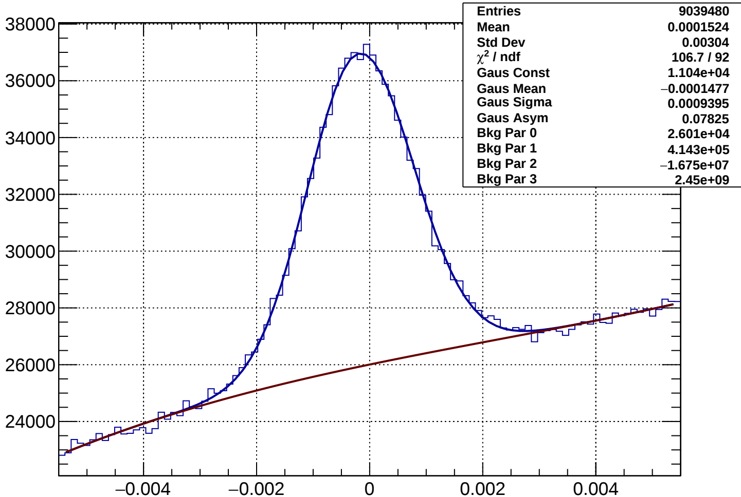
Rich1Gas proton Rec-Exp CKtheta - Bin 29 Ptot 35.155 to 36.35 GeV
