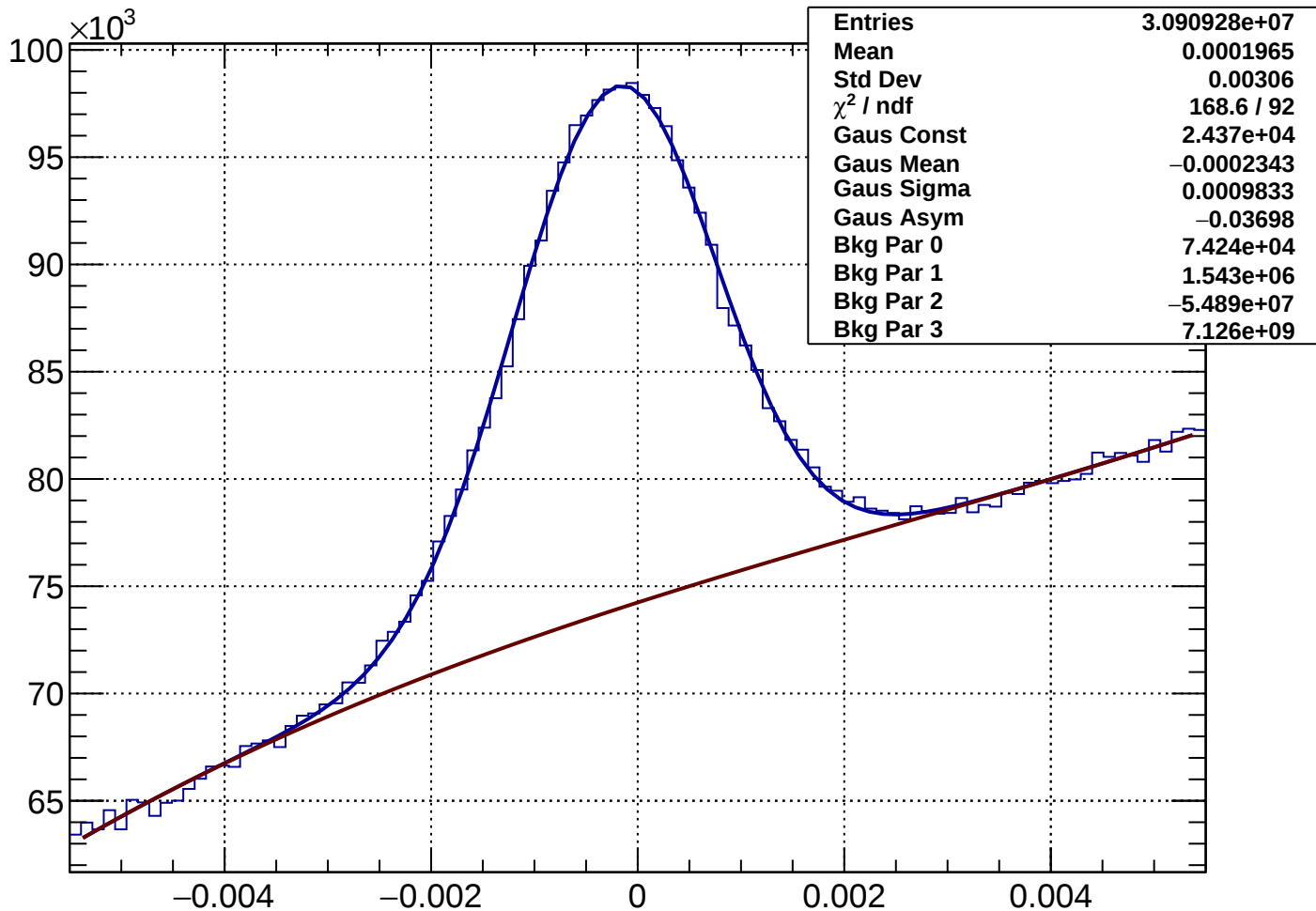
Rich1Gas proton Rec-Exp CKtheta - Bin 20 Ptot 24.4 to 25.595 GeV
