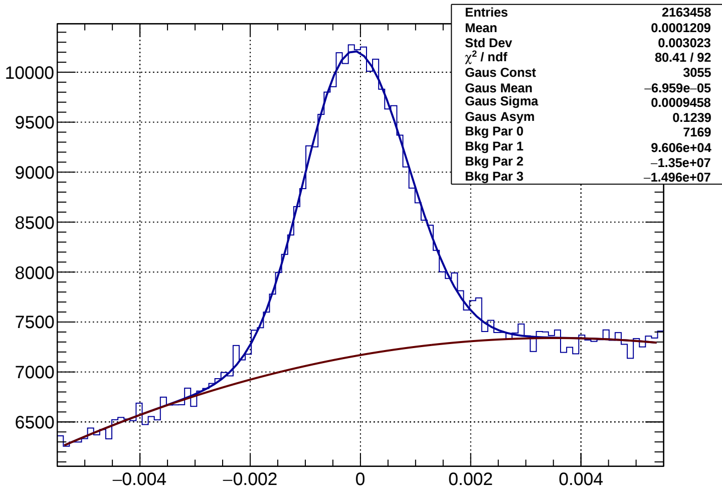
Rich1Gas proton Rec-Exp CKtheta - Bin 43 Ptot 51.885 to 53.08 GeV
