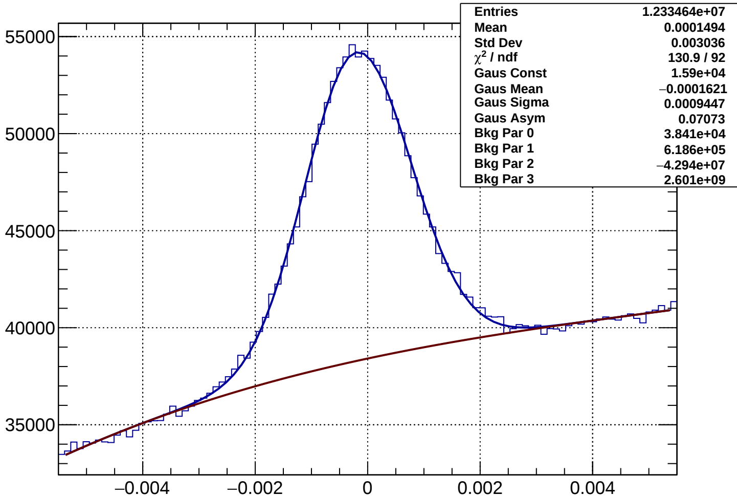
Rich1Gas proton Rec-Exp CKtheta - Bin 25 Ptot 30.375 to 31.57 GeV
