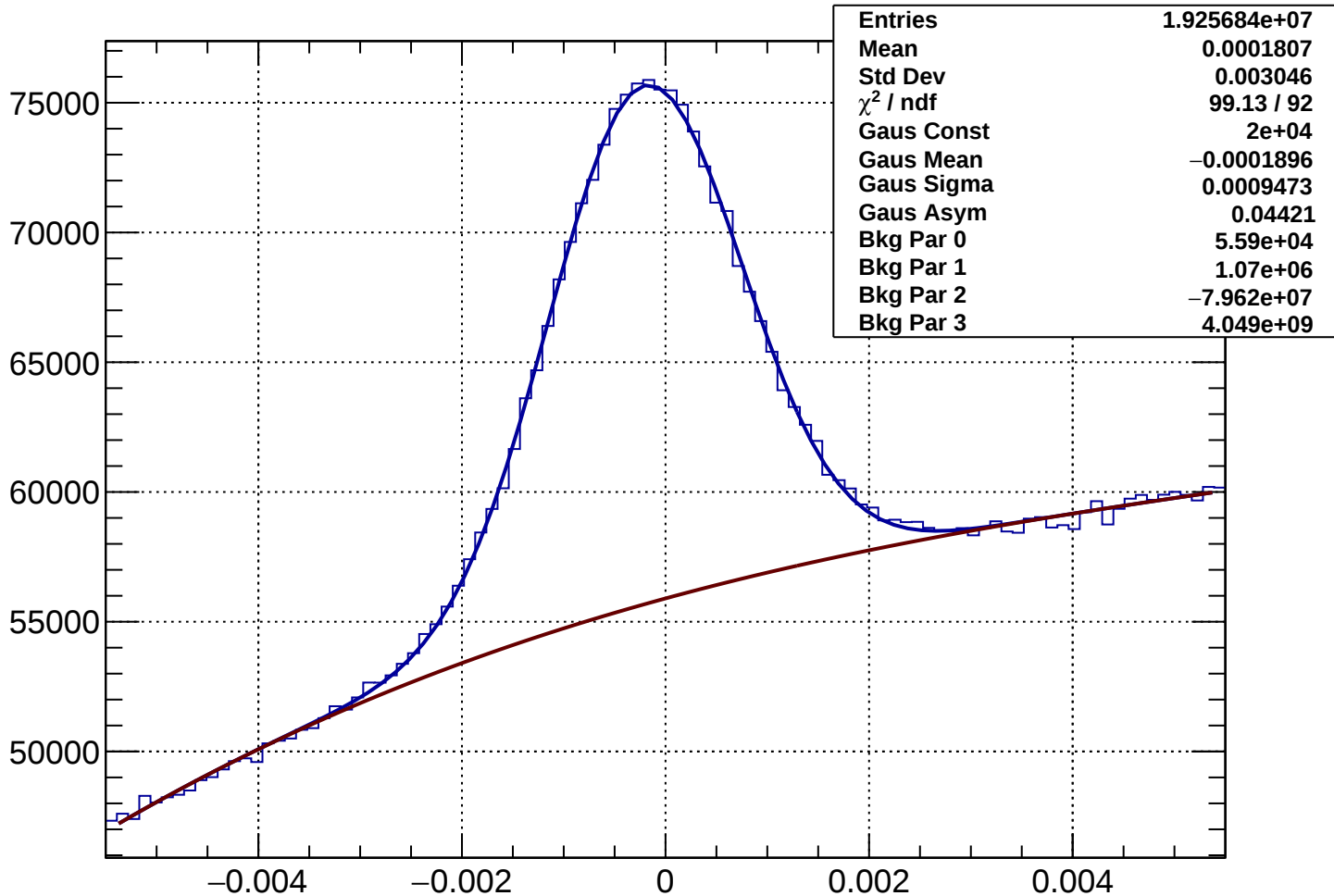
Rich1Gas proton Rec-Exp CKtheta - Bin 23 Ptot 27.985 to 29.18 GeV
