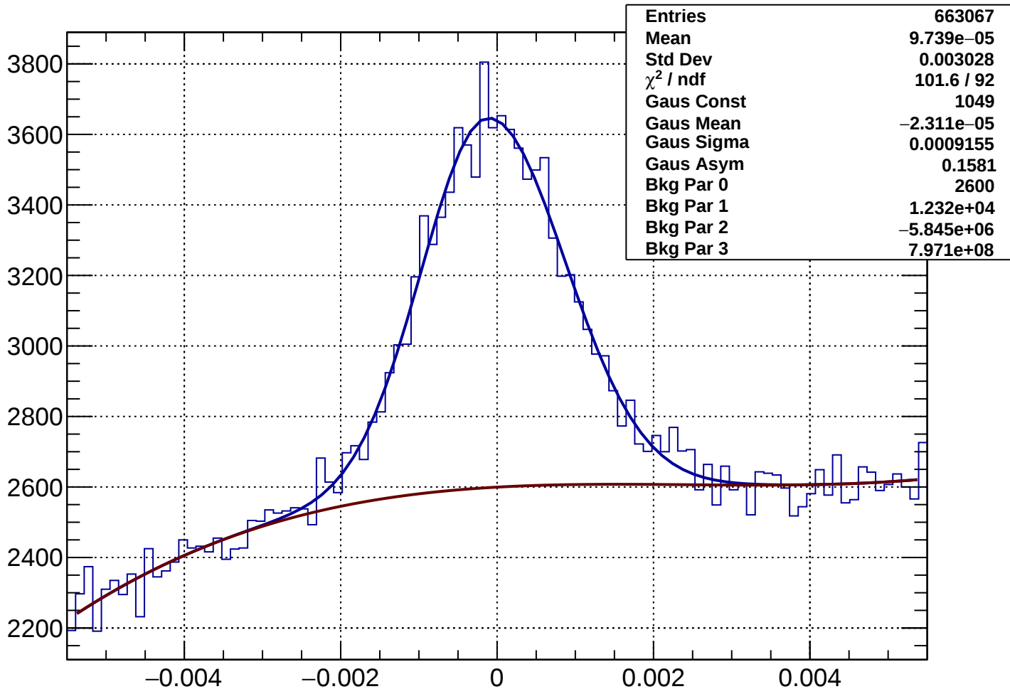
Rich1Gas proton Rec-Exp CKtheta - Bin 59 Ptot 71.005 to 72.2 GeV
