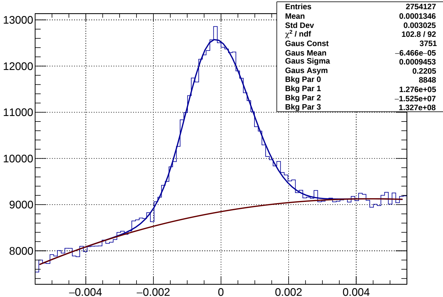
Rich1Gas proton Rec-Exp CKtheta - Bin 41 Ptot 49.495 to 50.69 GeV
