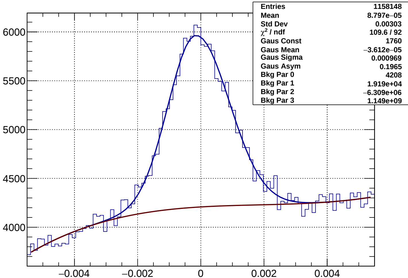
Rich1Gas proton Rec-Exp CKtheta - Bin 52 Ptot 62.64 to 63.835 GeV
