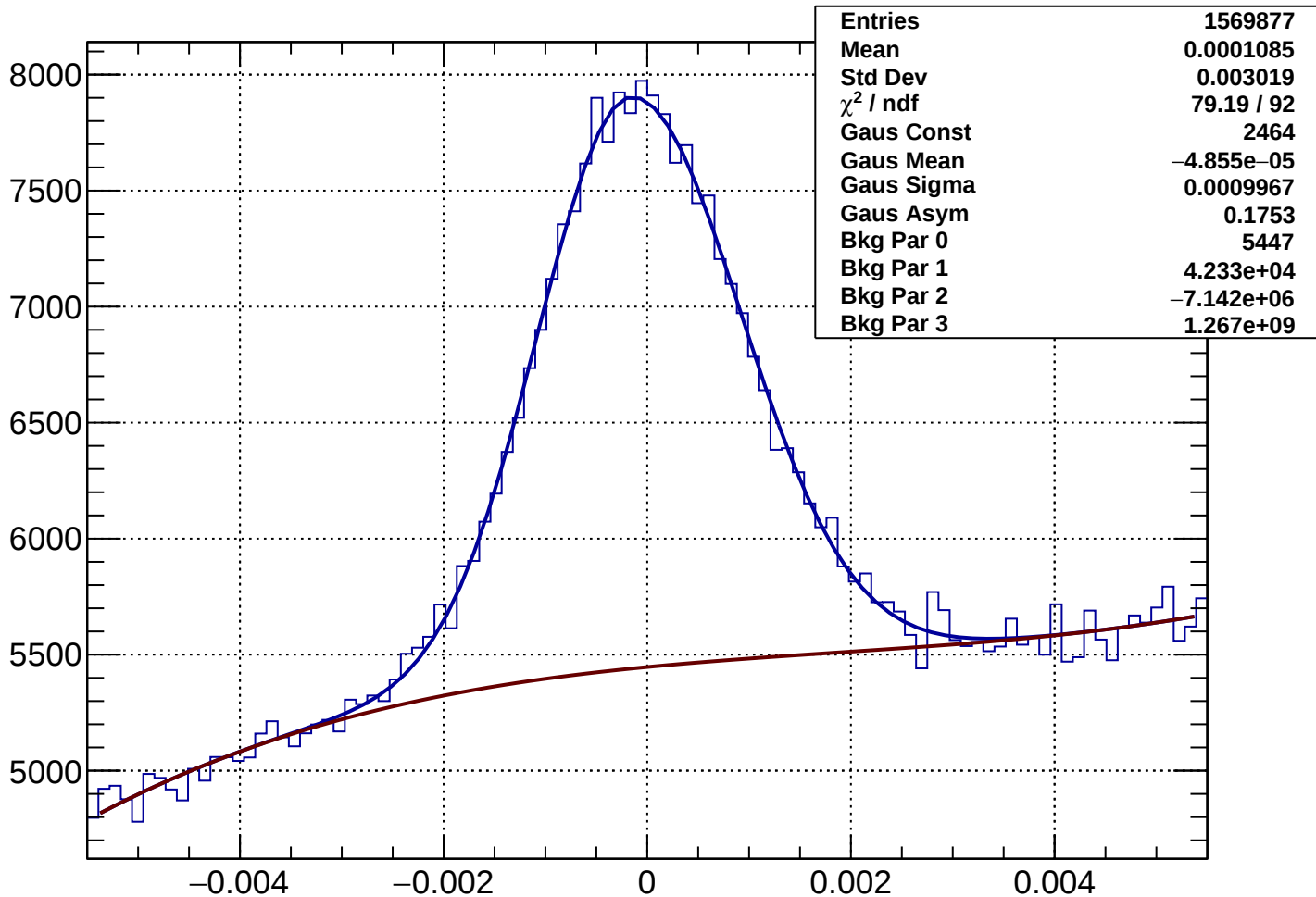
Rich1Gas proton Rec-Exp CKtheta - Bin 48 Ptot 57.86 to 59.055 GeV
