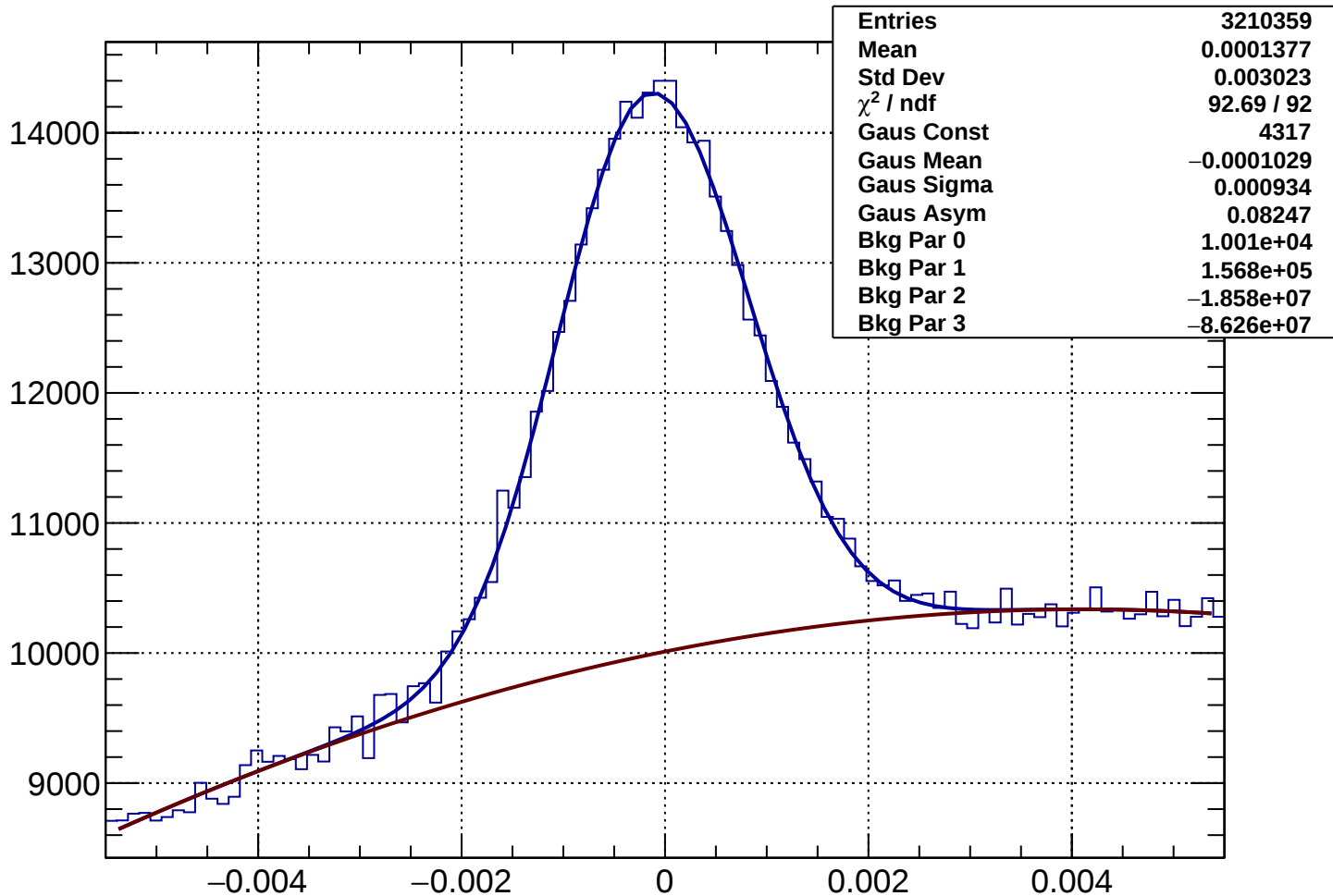
Rich1Gas proton Rec-Exp CKtheta - Bin 39 Ptot 47.105 to 48.3 GeV
