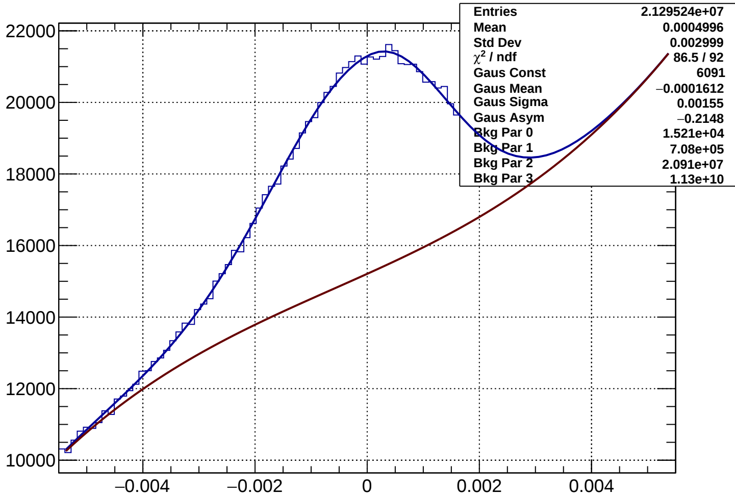
Rich1Gas proton Rec-Exp CKtheta - Bin 14 Ptot 17.23 to 18.425 GeV
