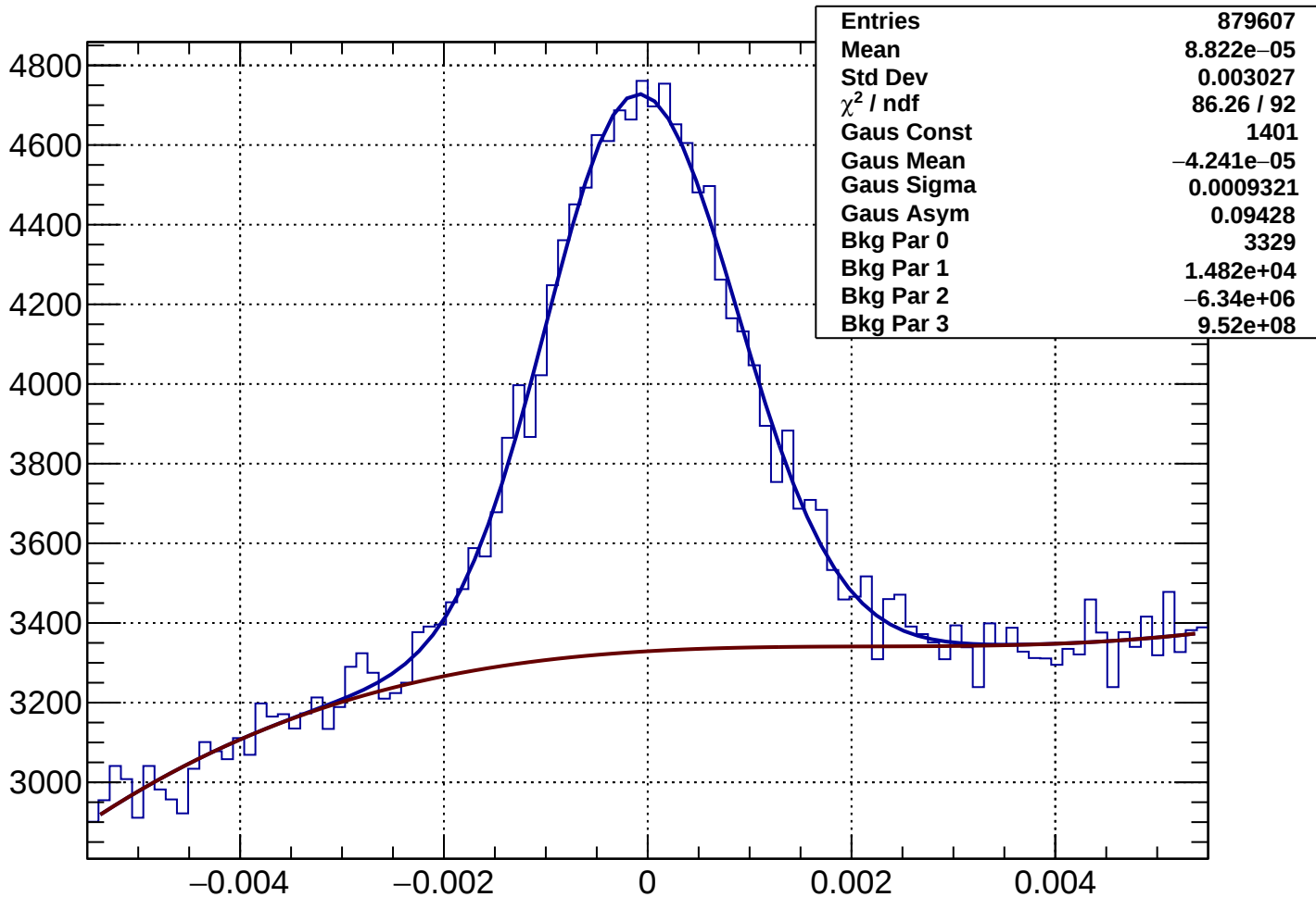
Rich1Gas proton Rec-Exp CKtheta - Bin 55 Ptot 66.225 to 67.42 GeV
