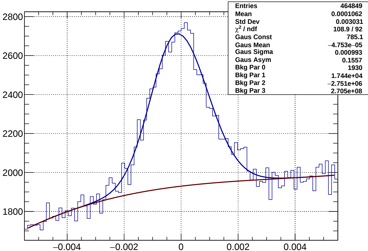
Rich1Gas proton Rec-Exp CKtheta - Bin 76 Ptot 91.32 to 92.515 GeV
