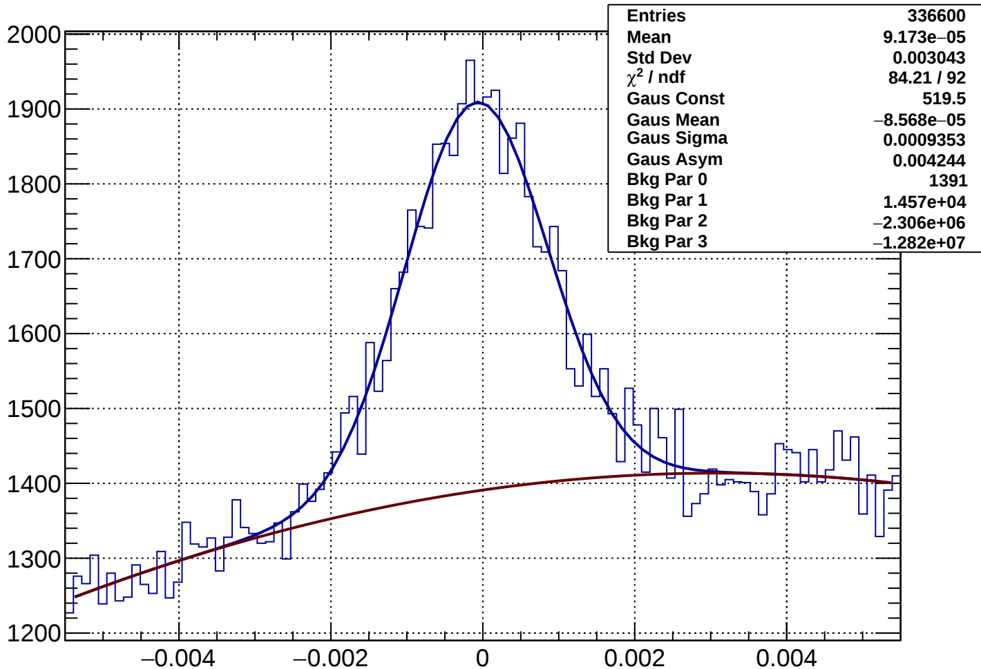
Rich1Gas proton Rec-Exp CKtheta - Bin 70 Ptot 84.15 to 85.345 GeV
