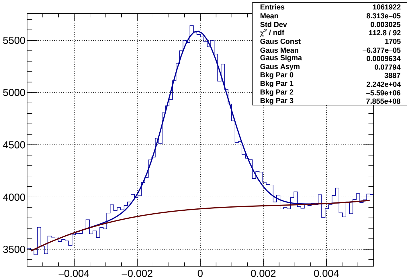
Rich1Gas proton Rec-Exp CKtheta - Bin 53 Ptot 63.835 to 65.03 GeV
