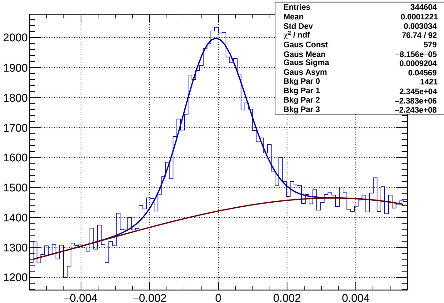
Rich1Gas proton Rec-Exp CKtheta - Bin 69 Ptot 82.955 to 84.15 GeV
