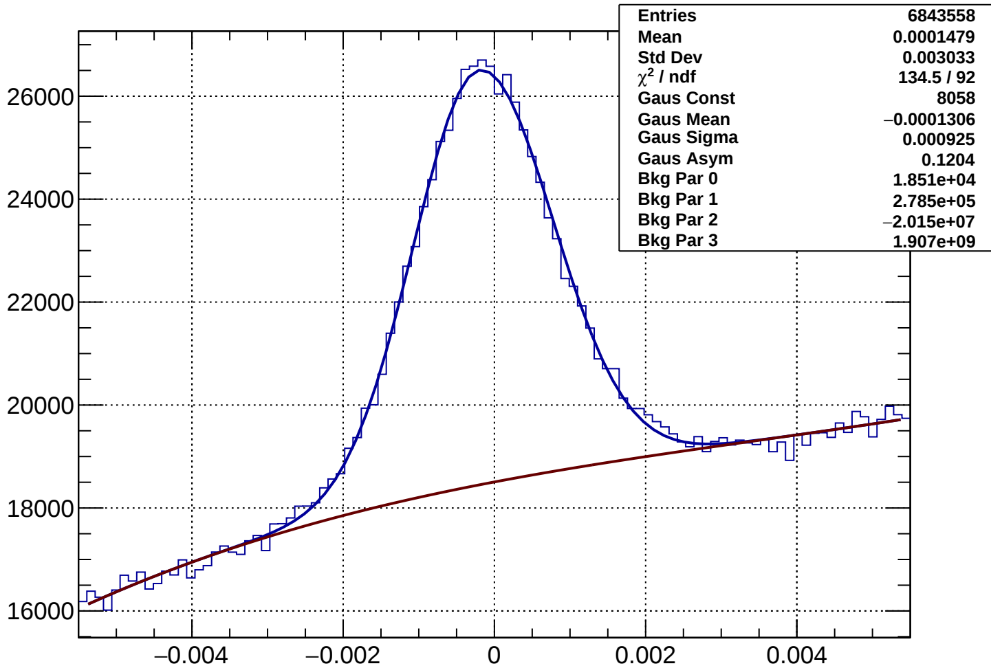
Rich1Gas proton Rec-Exp CKtheta - Bin 32 Ptot 38.74 to 39.935 GeV
