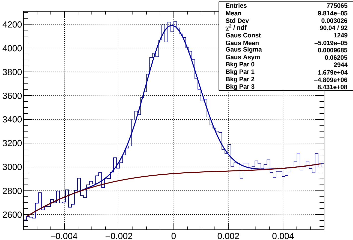
Rich1Gas proton Rec-Exp CKtheta - Bin 57 Ptot 68.615 to 69.81 GeV
