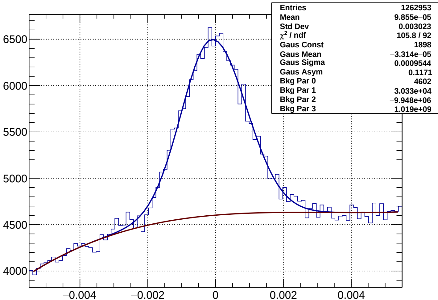
Rich1Gas proton Rec-Exp CKtheta - Bin 51 Ptot 61.445 to 62.64 GeV
