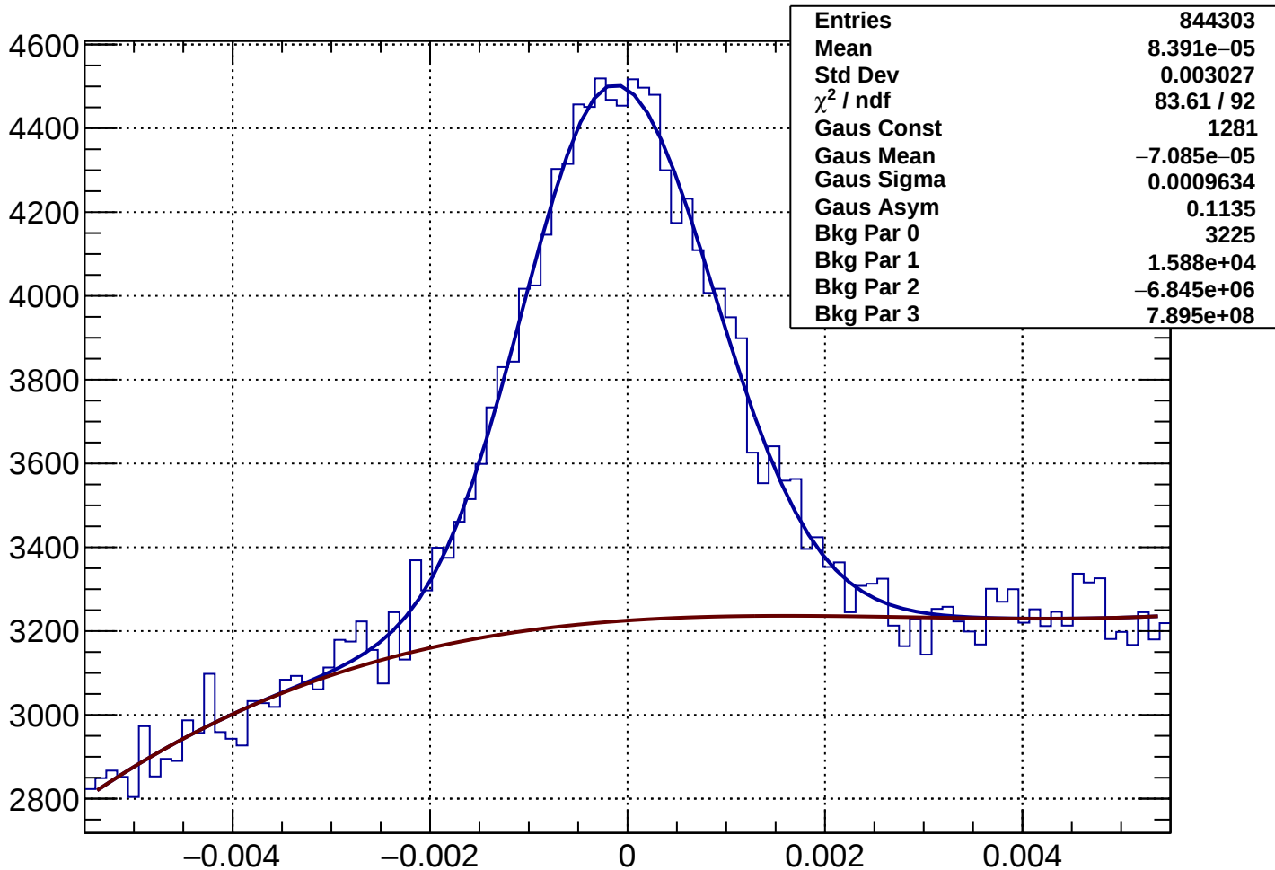
Rich1Gas proton Rec-Exp CKtheta - Bin 56 Ptot 67.42 to 68.615 GeV
