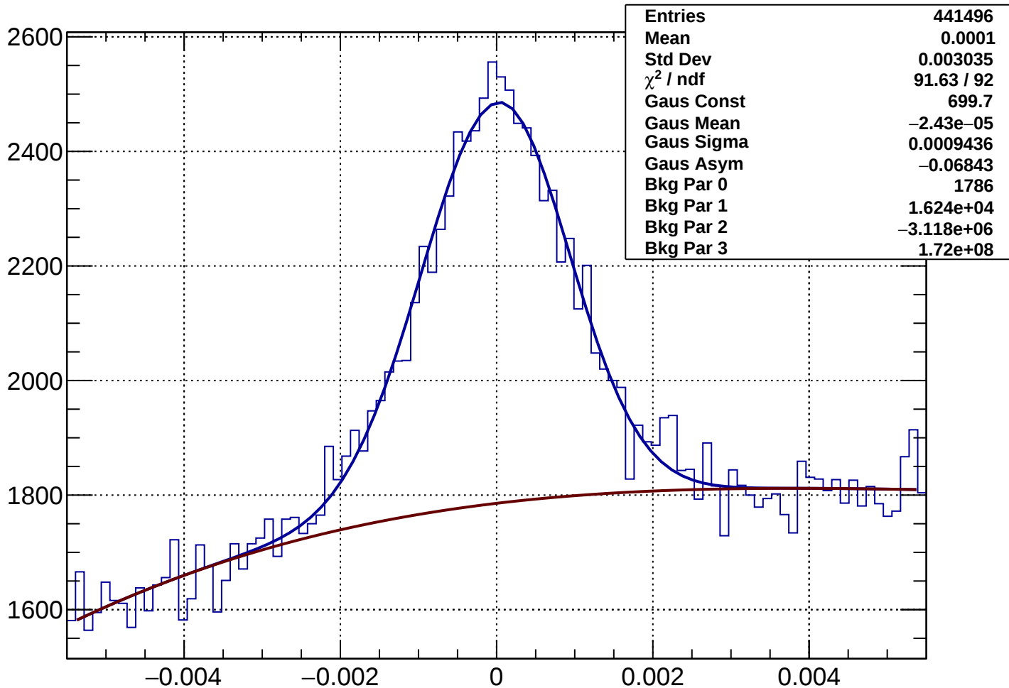
Rich1Gas proton Rec-Exp CKtheta - Bin 65 Ptot 78.175 to 79.37 GeV
