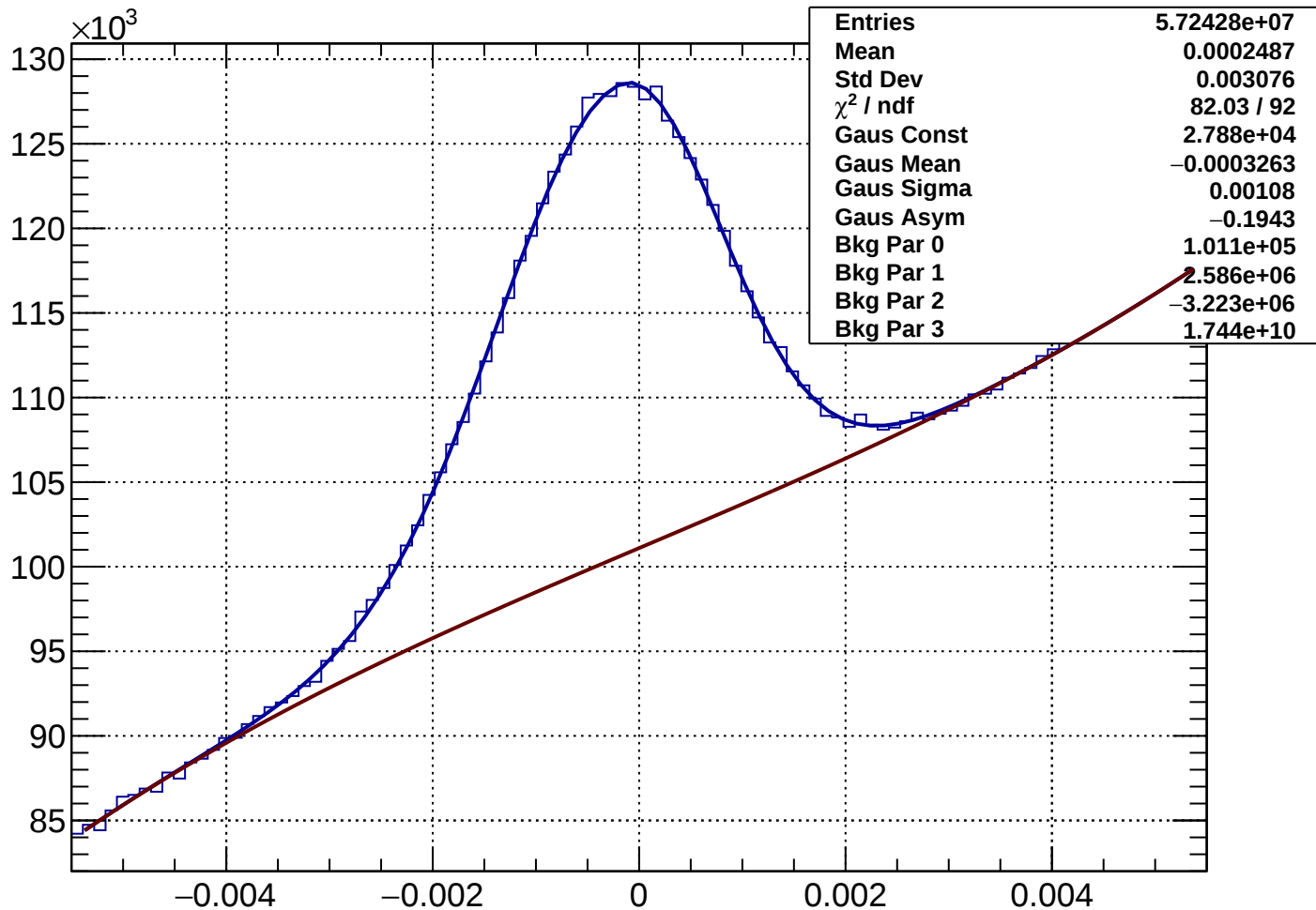
Rich1Gas proton Rec-Exp CKtheta - Bin 17 Ptot 20.815 to 22.01 GeV
