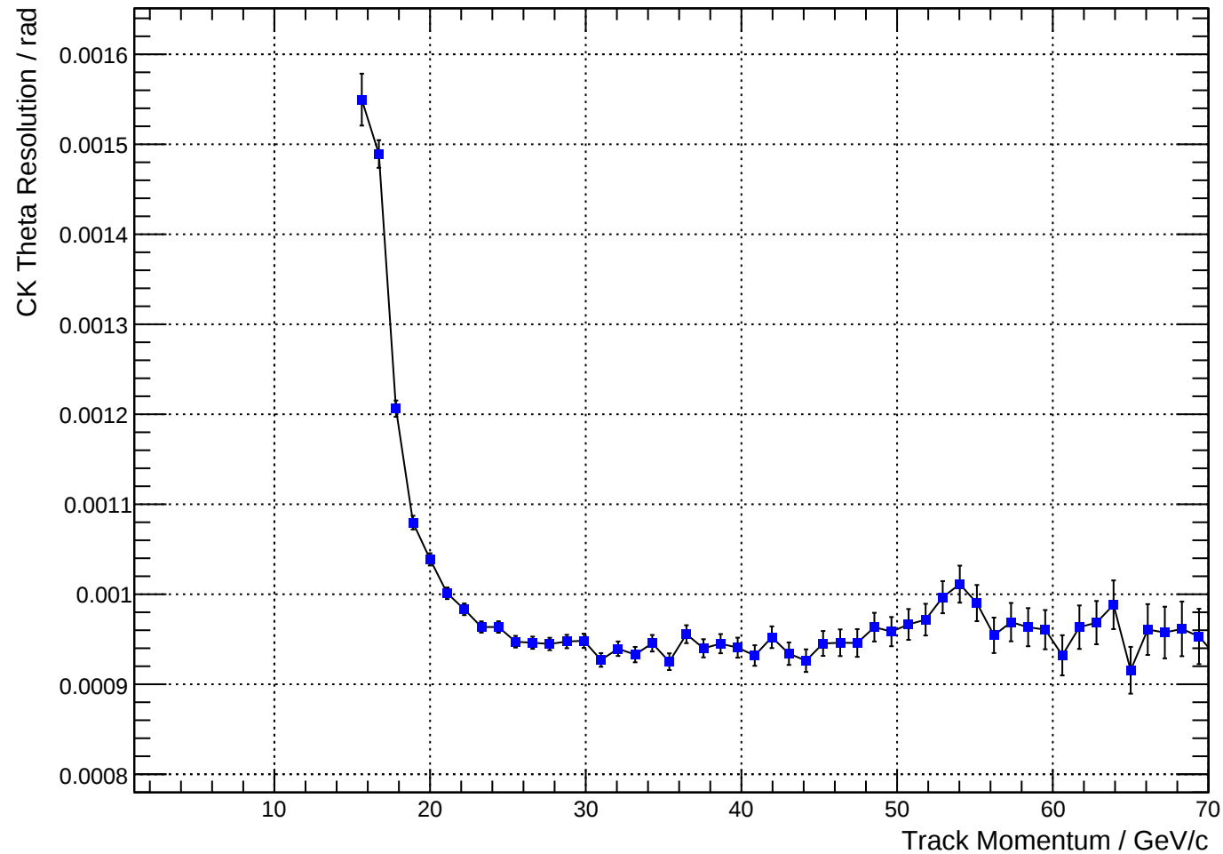
Rich1Gas Both proton CK Theta Resolution Versus Momentum
