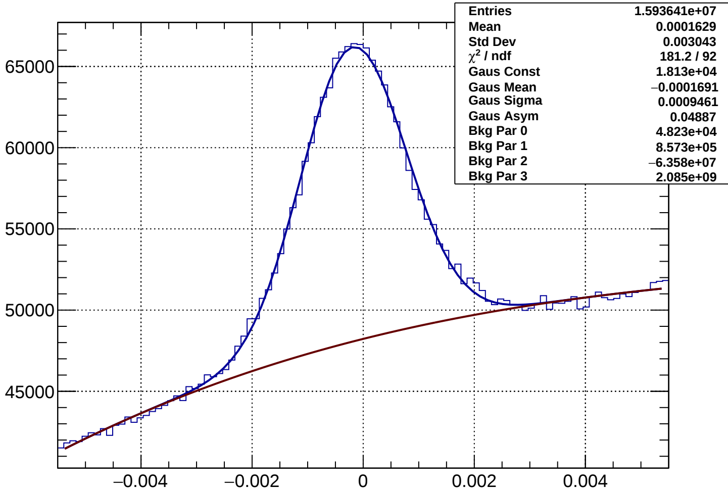
Rich1Gas proton Rec-Exp CKtheta - Bin 24 Ptot 29.18 to 30.375 GeV
