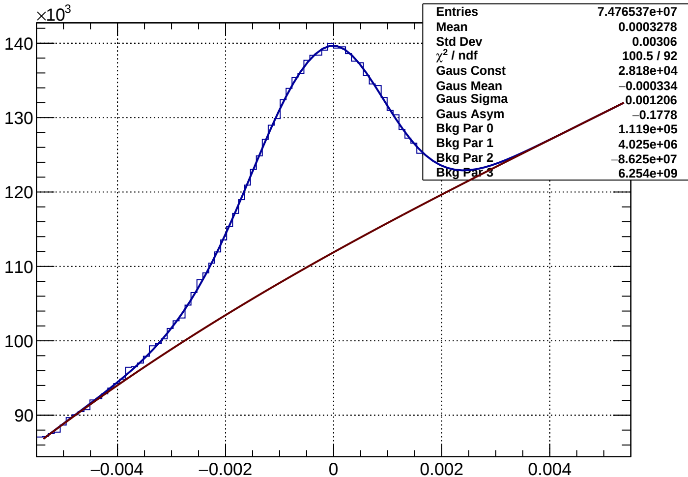
Rich1Gas proton Rec-Exp CKtheta - Bin 16 Ptot 19.62 to 20.815 GeV
