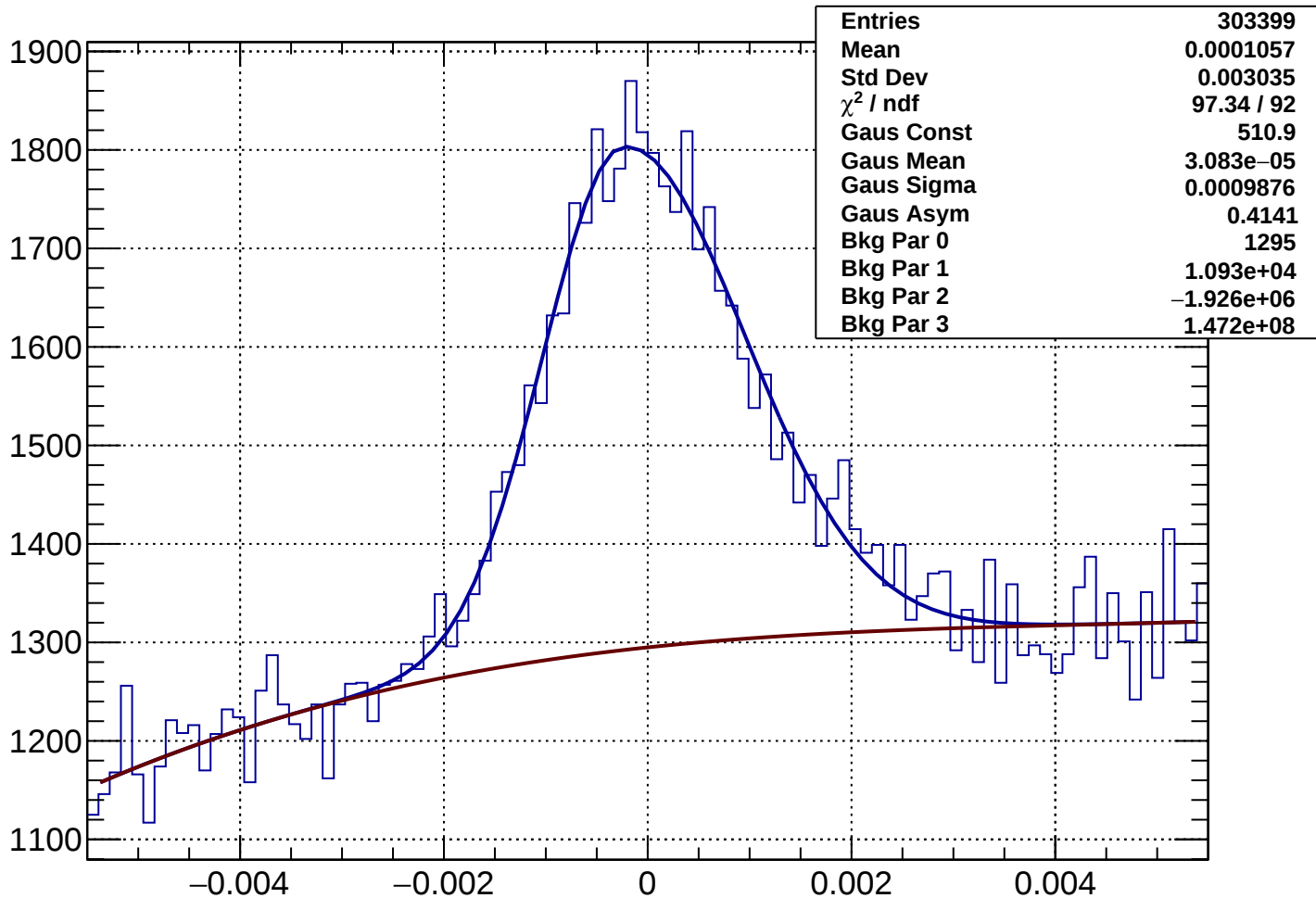
Rich1Gas proton Rec-Exp CKtheta - Bin 84 Ptot 100.88 to 102.075 GeV
