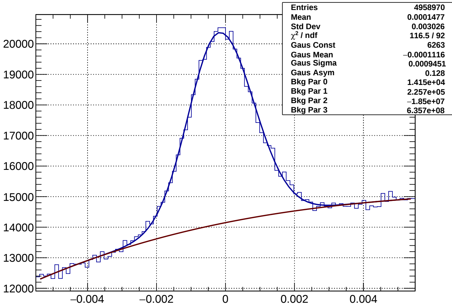
Rich1Gas proton Rec-Exp CKtheta - Bin 35 Ptot 42.325 to 43.52 GeV
