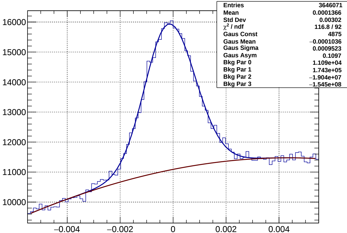
Rich1Gas proton Rec-Exp CKtheta - Bin 38 Ptot 45.91 to 47.105 GeV
