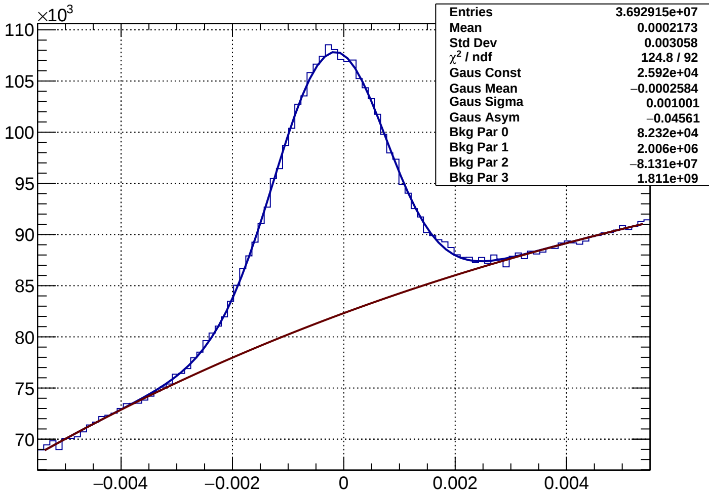
Rich1Gas proton Rec-Exp CKtheta - Bin 19 Ptot 23.205 to 24.4 GeV
