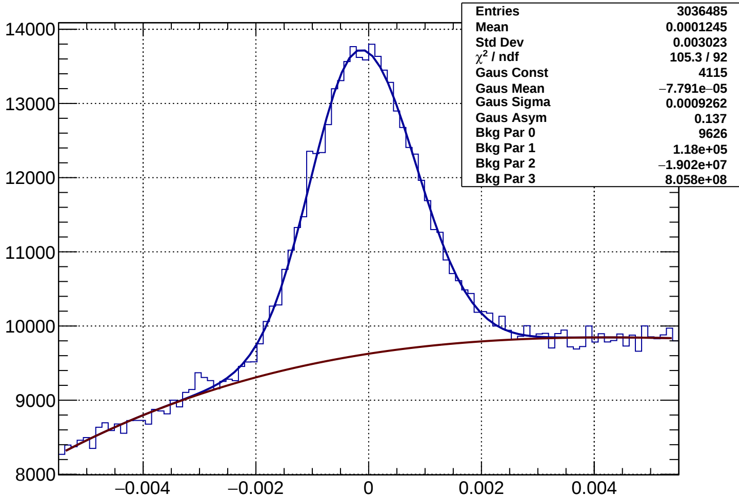
Rich1Gas proton Rec-Exp CKtheta - Bin 40 Ptot 48.3 to 49.495 GeV
