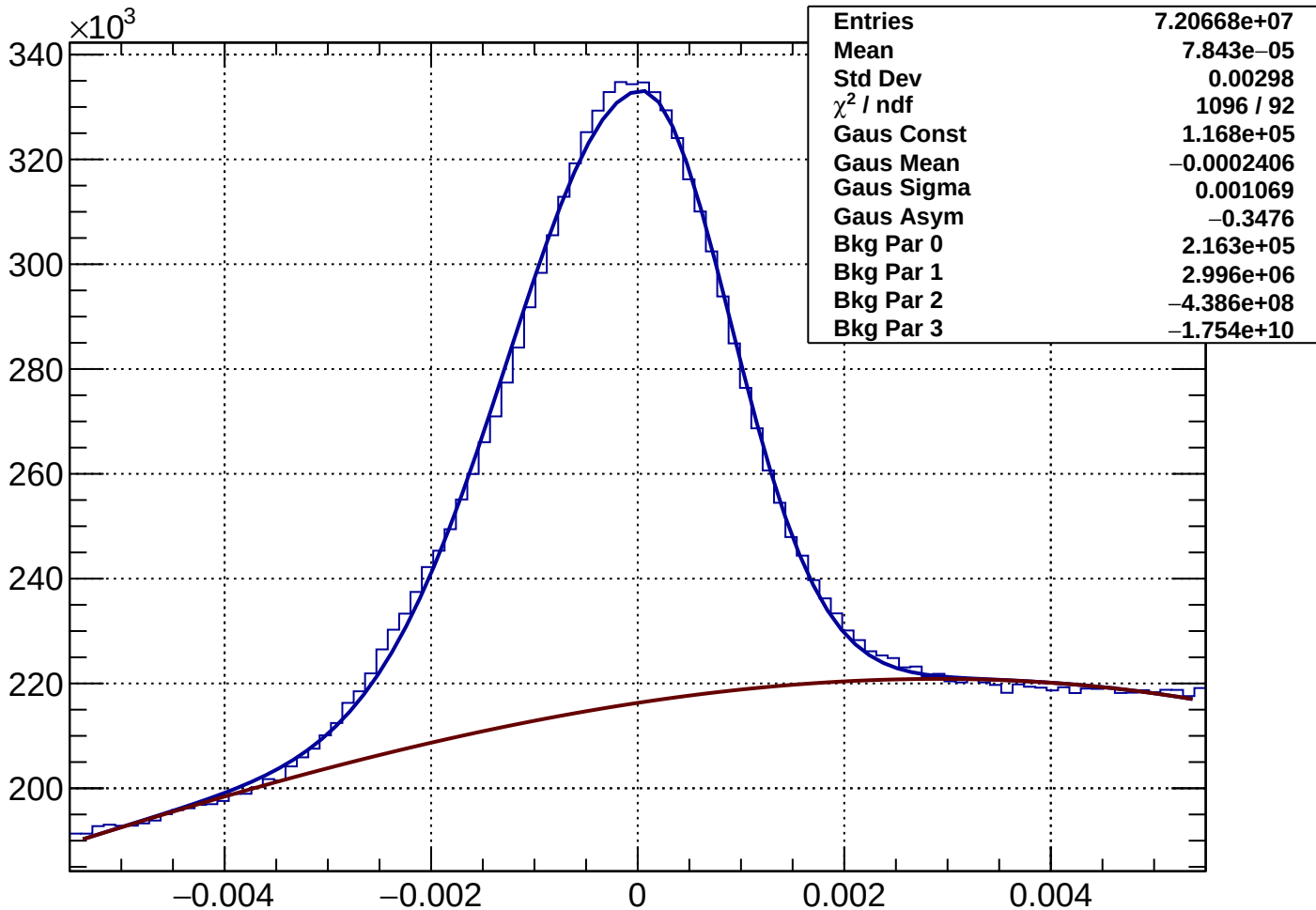
Rich1Gas muon Rec-Exp CKtheta - Bin 7 Ptot 8.865 to 10.06 GeV
