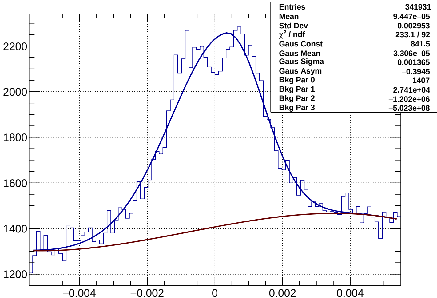
Rich1Gas muon Rec-Exp CKtheta - Bin 88 Ptot 105.66 to 106.855 GeV
