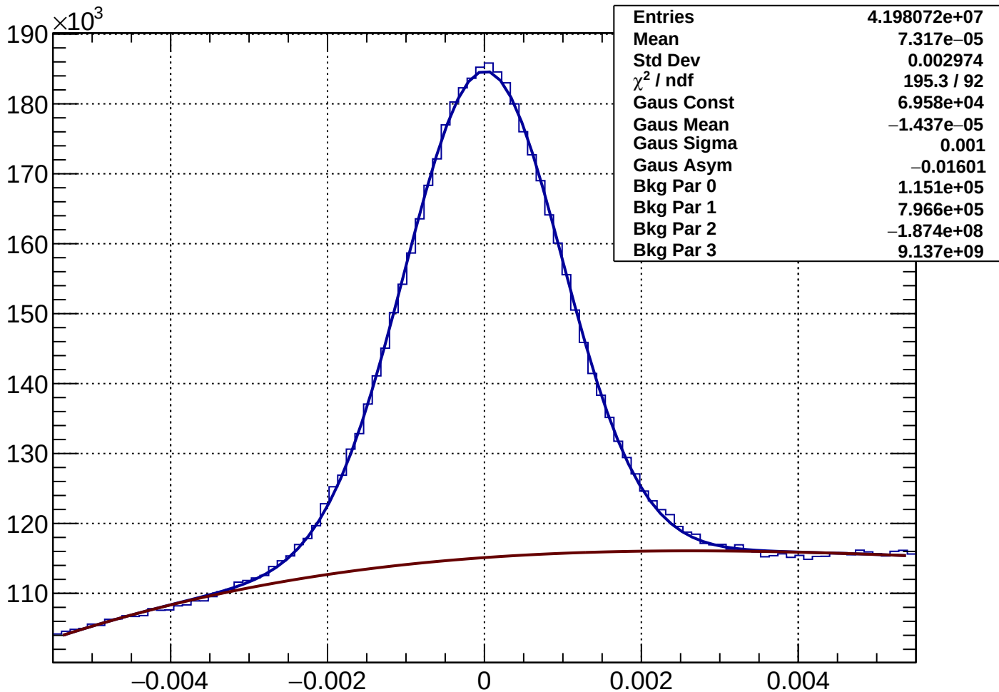
Rich1Gas muon Rec-Exp CKtheta - Bin 16 Ptot 19.62 to 20.815 GeV
