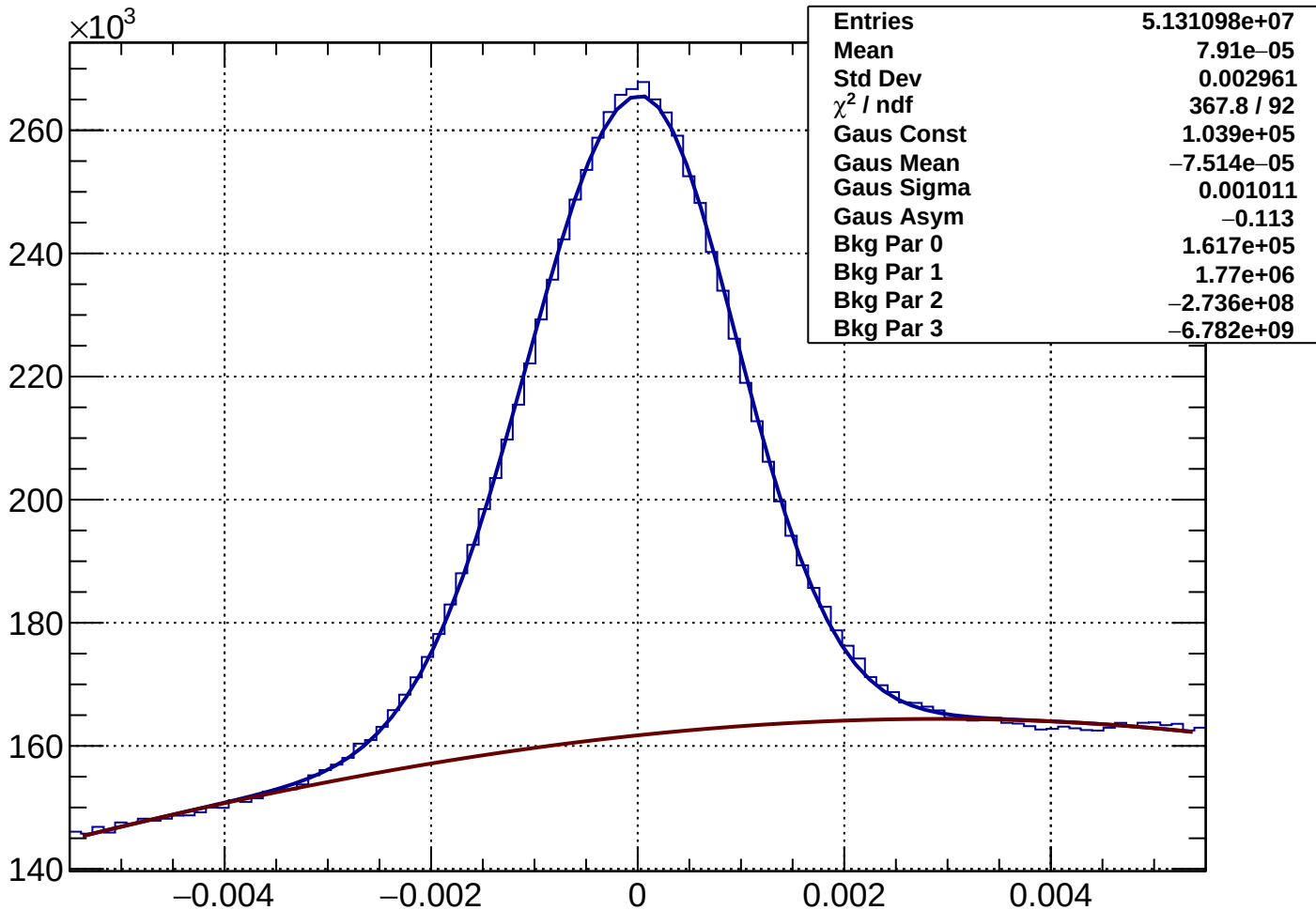
Rich1Gas muon Rec-Exp CKtheta - Bin 11 Ptot 13.645 to 14.84 GeV
