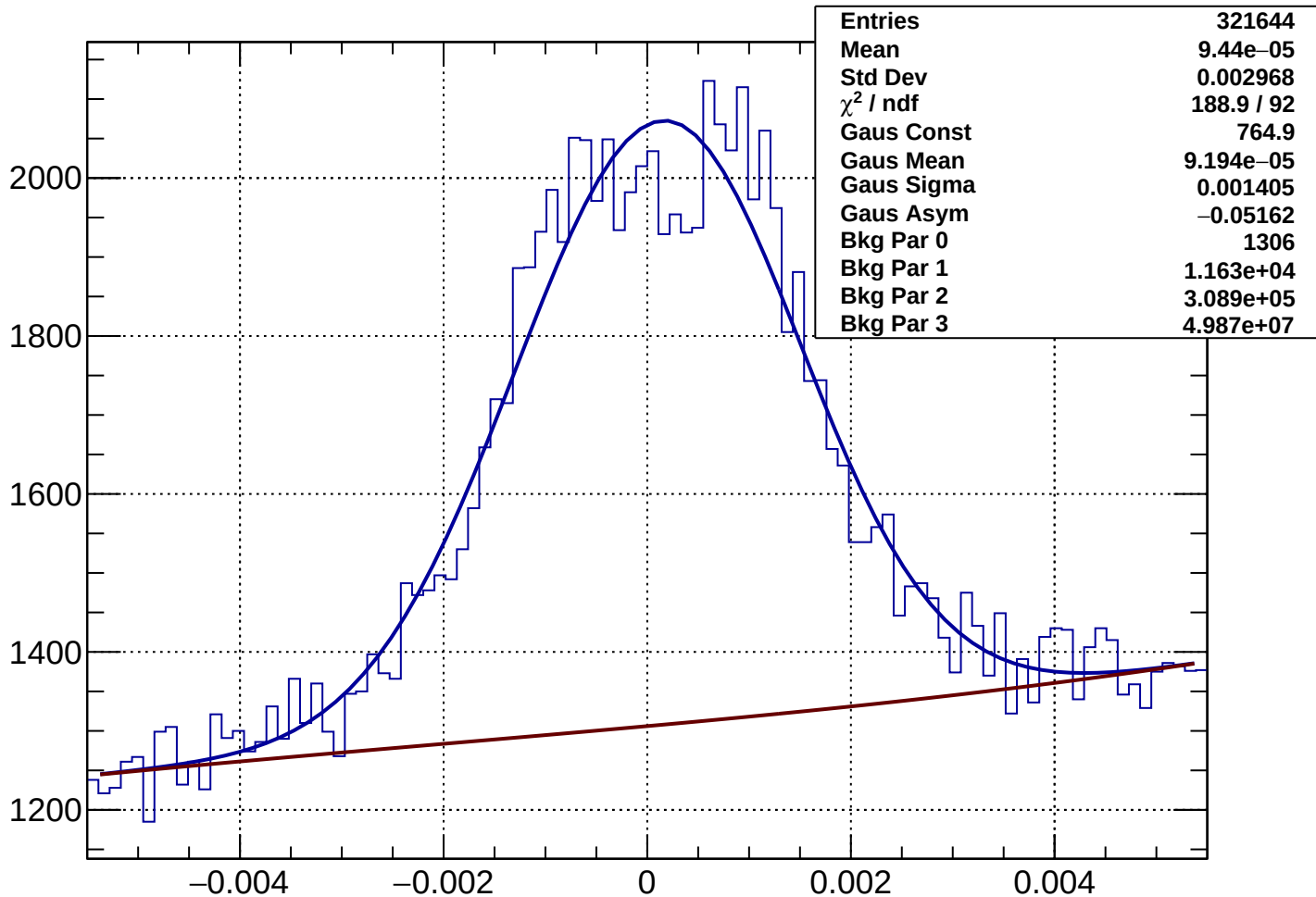
Rich1Gas muon Rec-Exp CKtheta - Bin 91 Ptot 109.245 to 110.44 GeV
