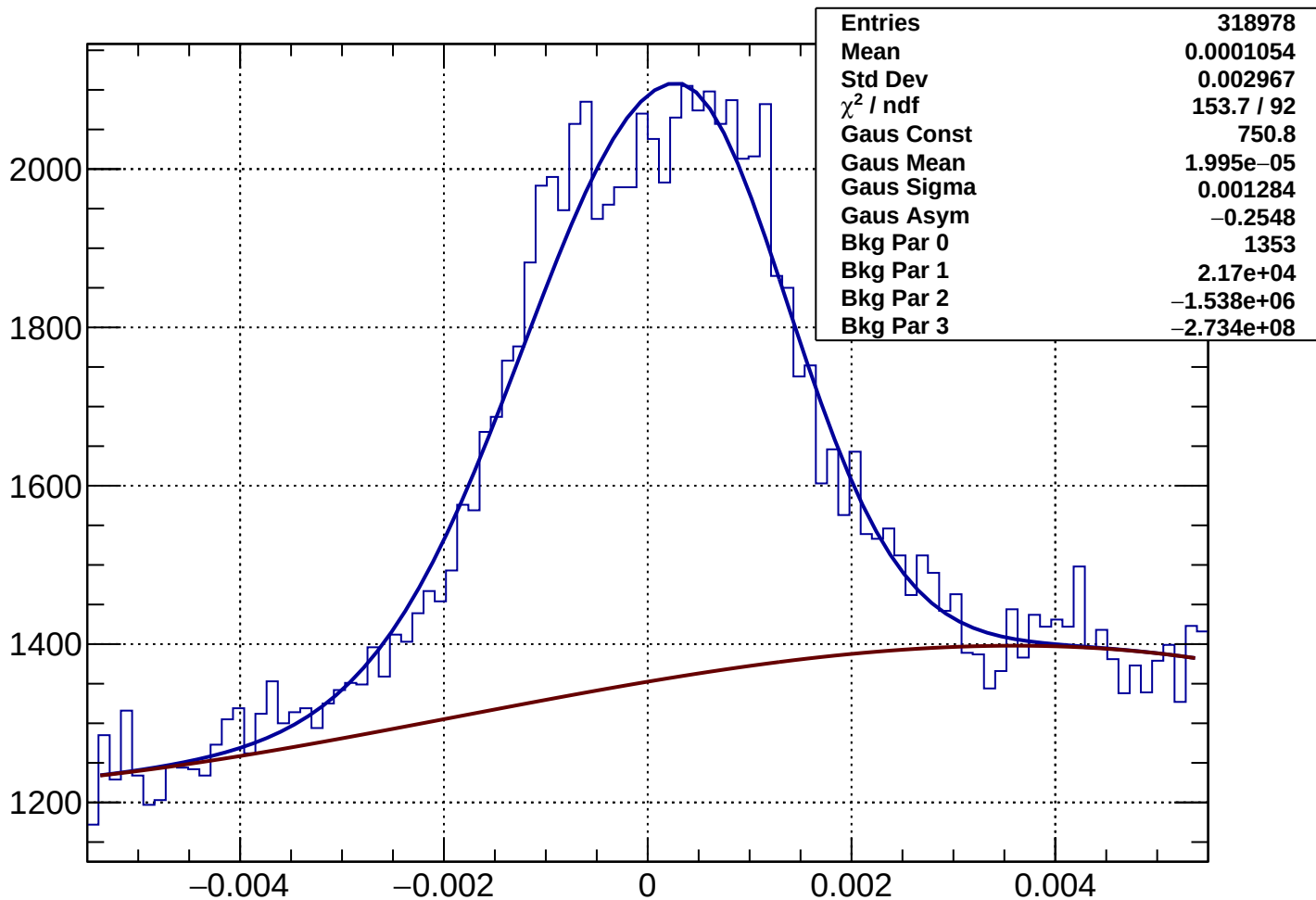
Rich1Gas muon Rec-Exp CKtheta - Bin 97 Ptot 116.415 to 117.61 GeV
