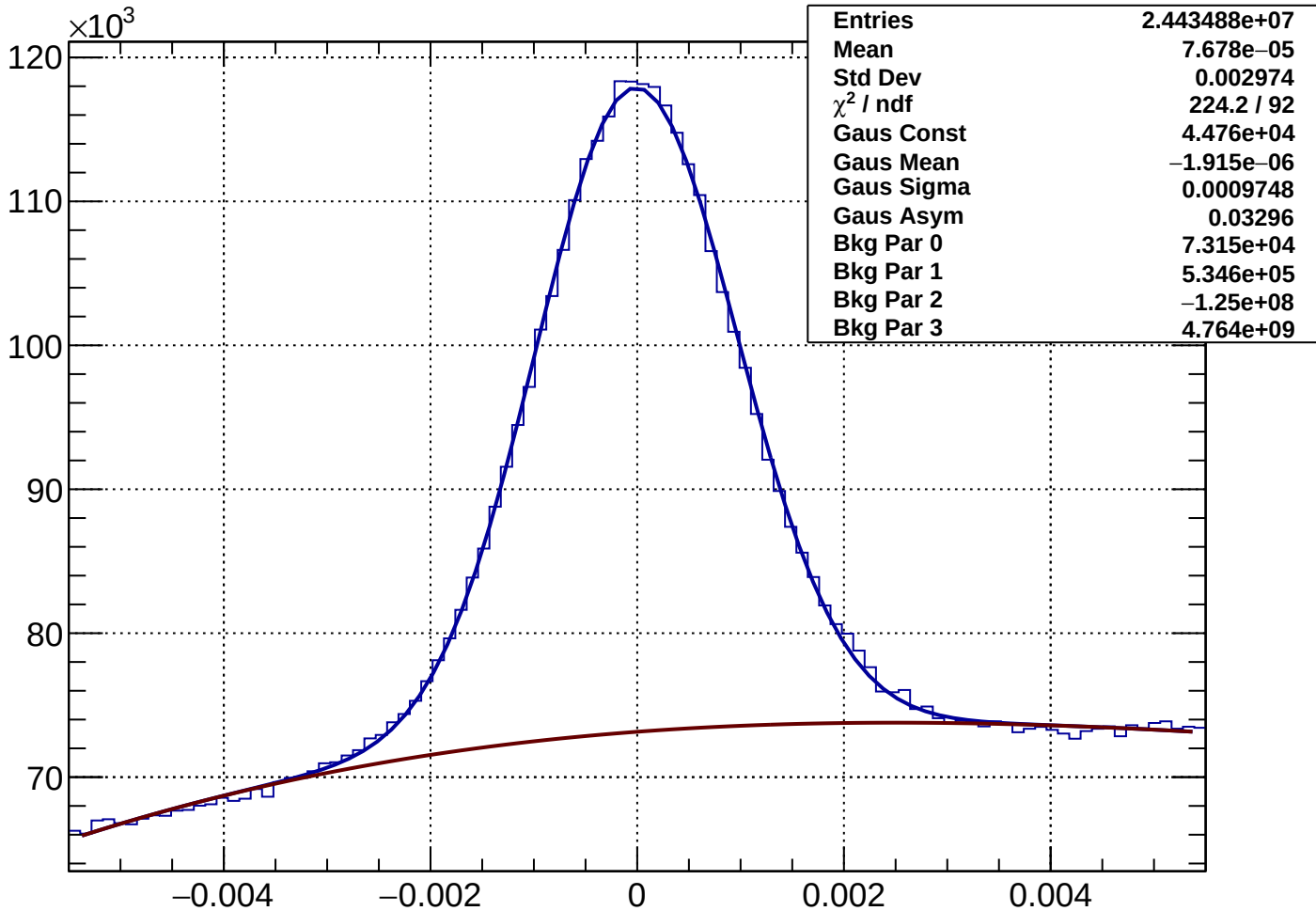
Rich1Gas muon Rec-Exp CKtheta - Bin 19 Ptot 23.205 to 24.4 GeV
