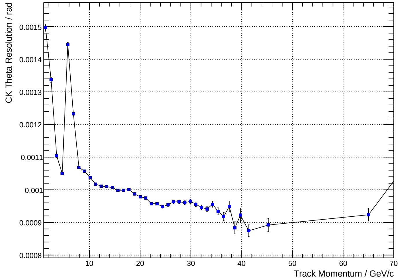
Rich1Gas Both muon CK Theta Resolution Versus Momentum
