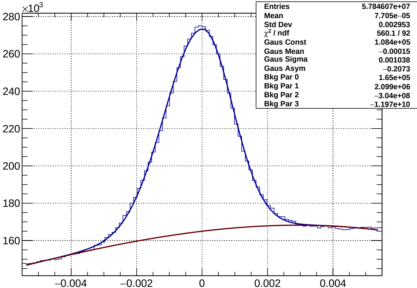
Rich1Gas muon Rec-Exp CKtheta - Bin 9 Ptot 11.255 to 12.45 GeV
