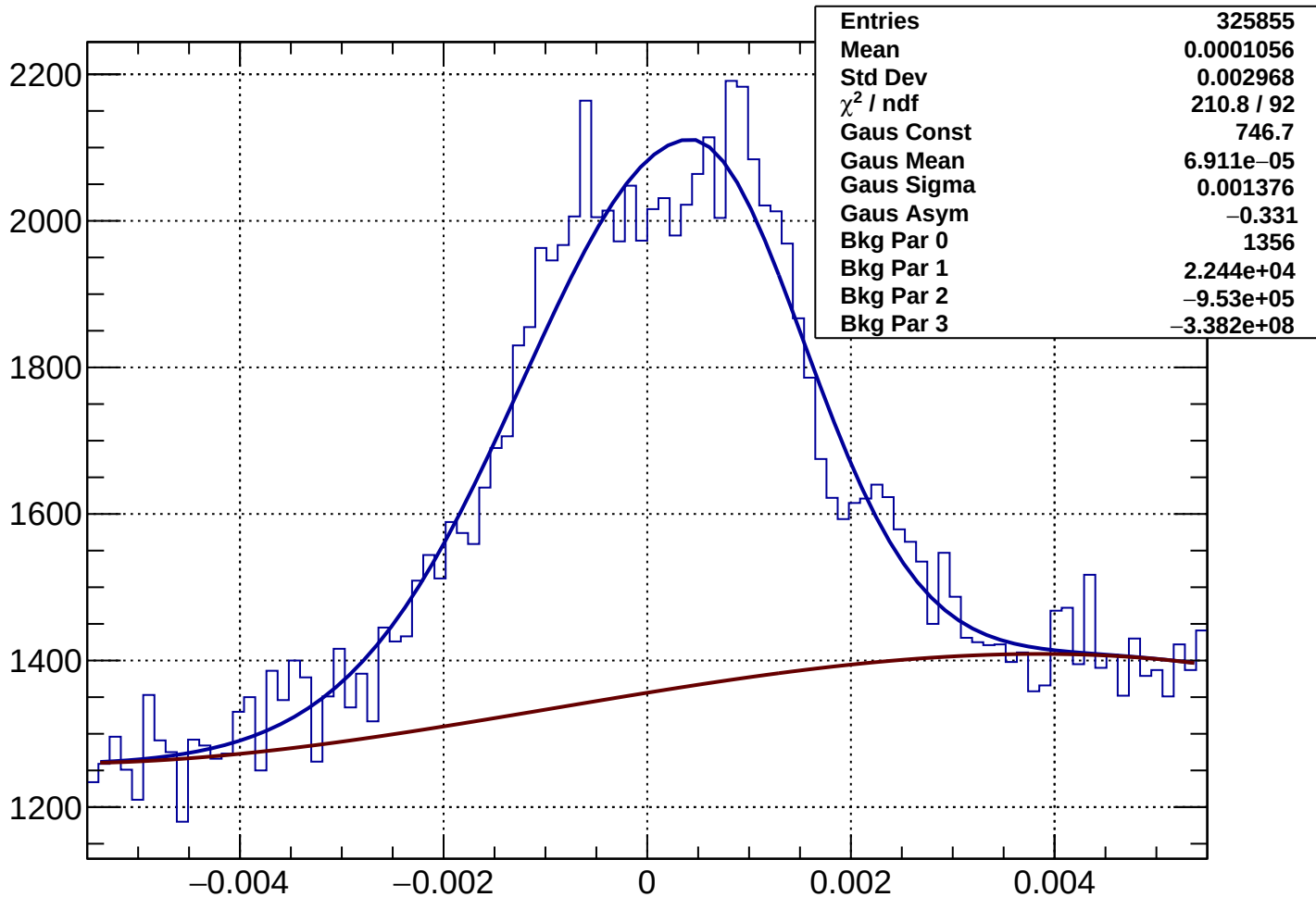
Rich1Gas muon Rec-Exp CKtheta - Bin 94 Ptot 112.83 to 114.025 GeV
