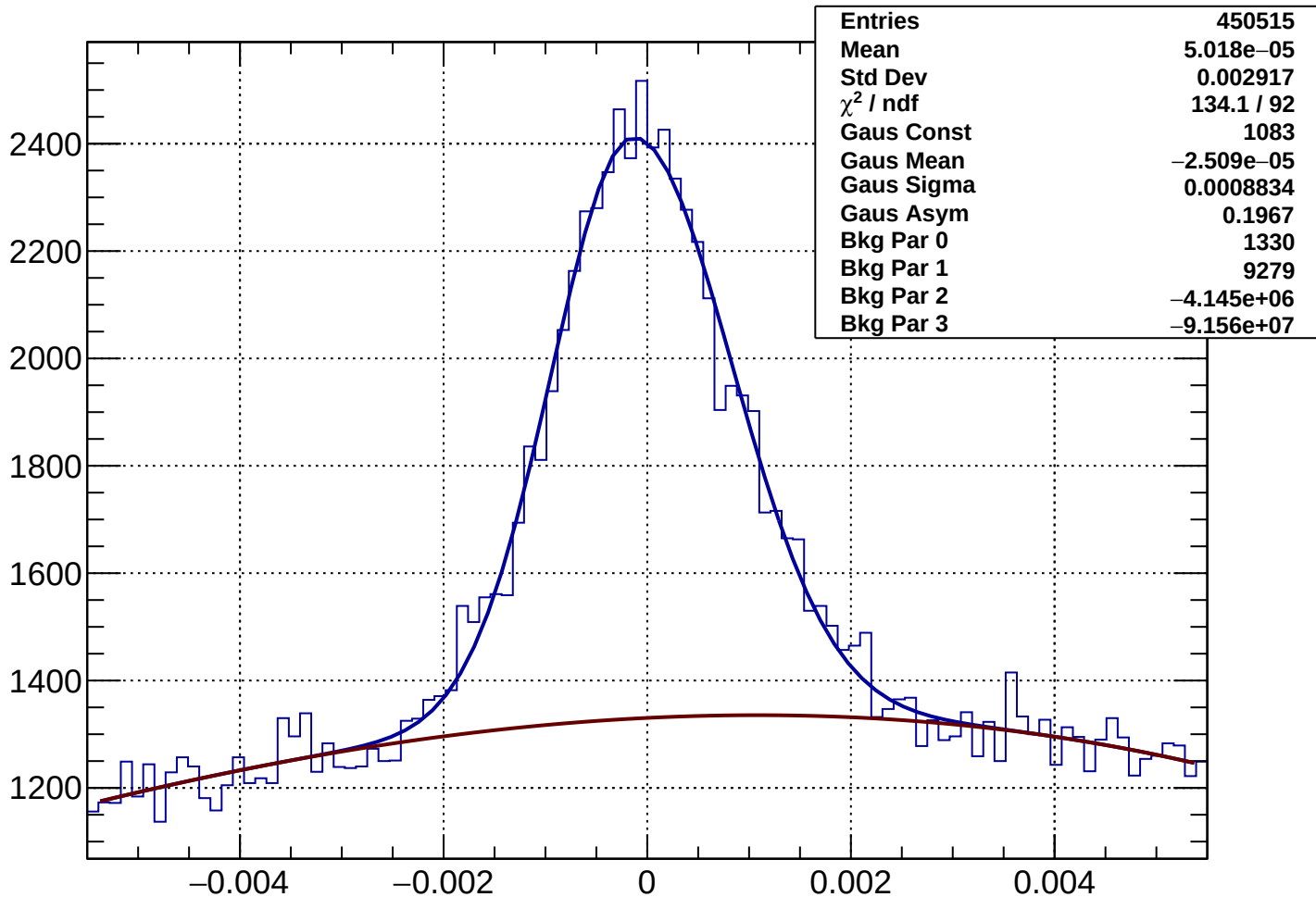
Rich1Gas muon Rec-Exp CKtheta - Bin 35 Ptot 42.325 to 43.52 GeV
