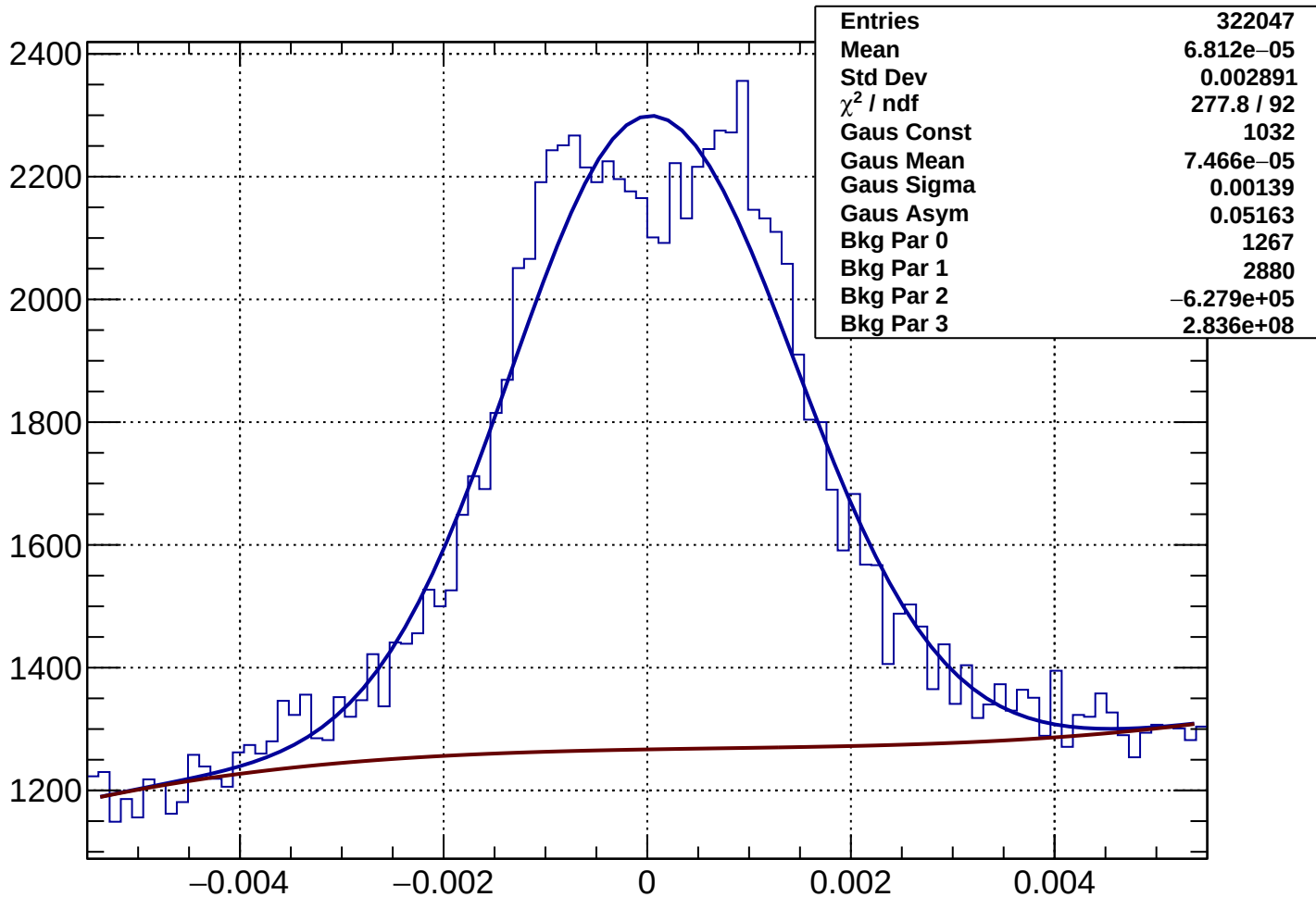
Rich1Gas muon Rec-Exp CKtheta - Bin 84 Ptot 100.88 to 102.075 GeV
