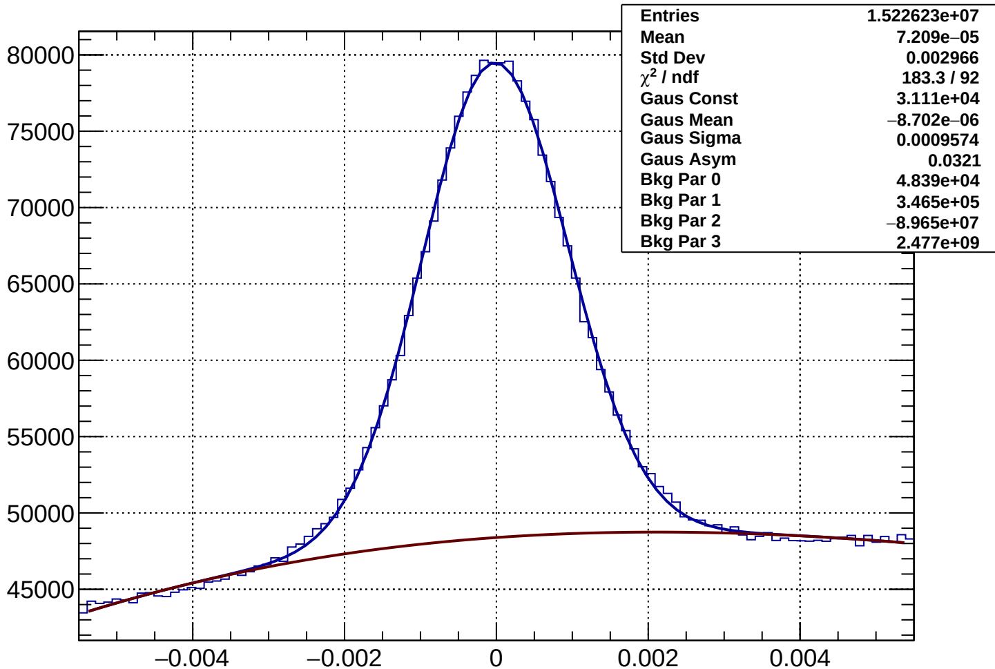
Rich1Gas muon Rec-Exp CKtheta - Bin 21 Ptot 25.595 to 26.79 GeV
