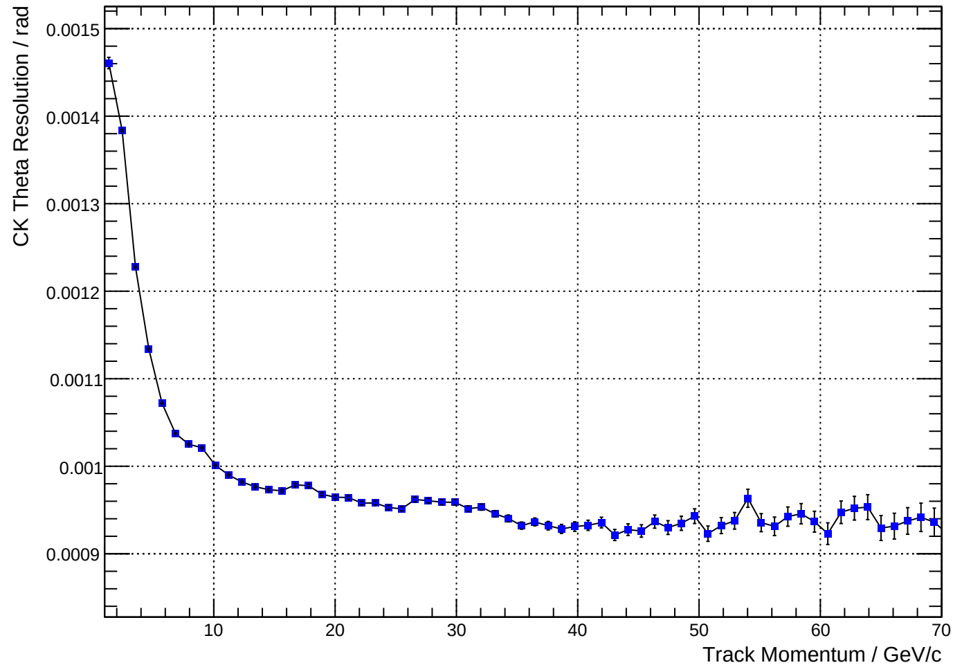
Rich1Gas Both All CK Theta Resolution Versus Momentum
