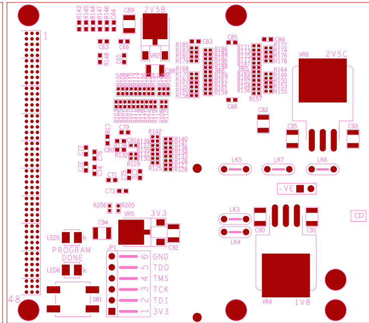
BOTTOM SILK SCREEN
