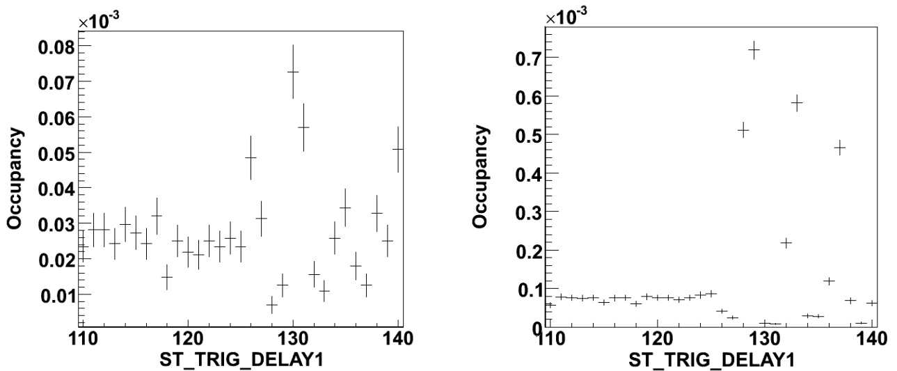
(a) A typical electrical noise pickup candidate. The occupancy increase at 126 and 130 bunch-crossings precede any optical activity.
