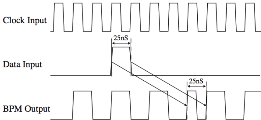
Figure 2-7: The principle of bi-phase mark(BPM) encoding,[41]. BPM combines clock and command into one stream. A chain of 0's gives a 20 MHz clock. As illustrated, a 1 gives a flip of the clock phase. The BPM chip delays the signal by three bunch-crossings.
