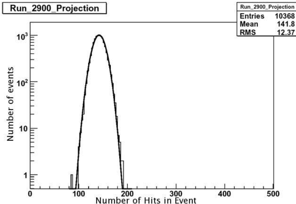
Figure 5-21: The occupancy of events histogram for a noise run for all 3 time-bins, [108], with a random trigger.
