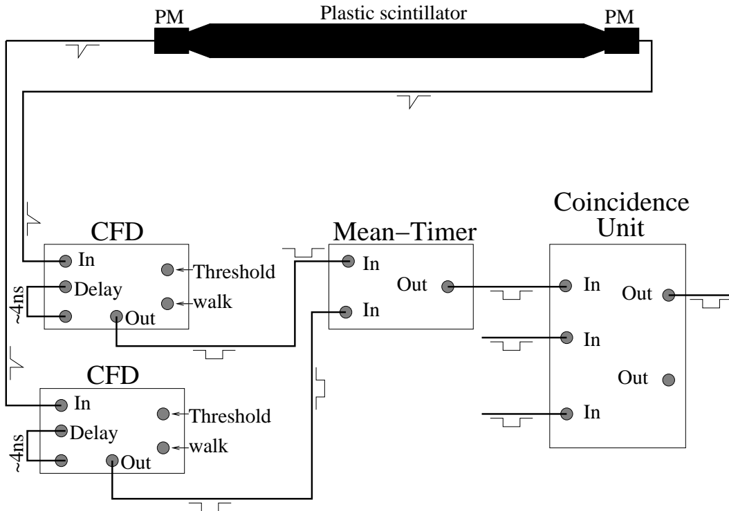
Figure 5-4: Schematic of the cosmic NIM trigger logic. Only one scintillator is shown. The trigger required a coincidence between the mean-timer outputs of the upper two scintillators shown in Fig. 5-3.
