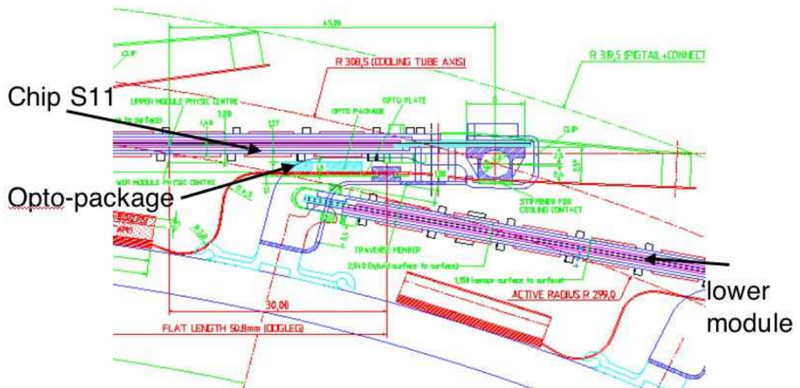
Figure 3-37: A barrel schematic in the r\text{-}\phi plane showing that the silicon strips corresponding to chip S11 of a module are right over that module's opto-package, explaining why chip S11 is most susceptible to light leaks.
