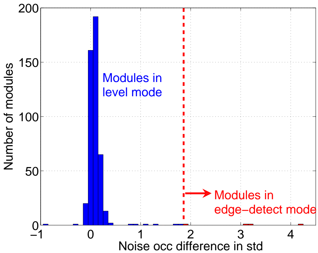
Figure 5-22: The histogram of the noise occupancy difference between physics and calibration mode in standard deviations for each module in the cosmics sector.
