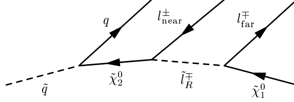
Figure 3: “Sequential” decay.
