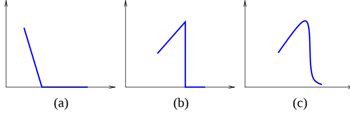
Figure 7: Line-shapes used for fits to the mass distributions. Shape (a) (or its reflection in the vertical axis) is the standard “straight line” used to extract the l^+l^-q edge, l^\pm q high-edge, l^\pm q low-edge and l^+l^-q threshold resolutions. Shape (b) models the expected shape of the sharp l^+l^- edge in the absence of detector effects. The l^+l^- edge is actually fitted with shape (c), which is identical to (b) except that it is smeared with a gaussian resolution whose width is a free parameter of the fit.
