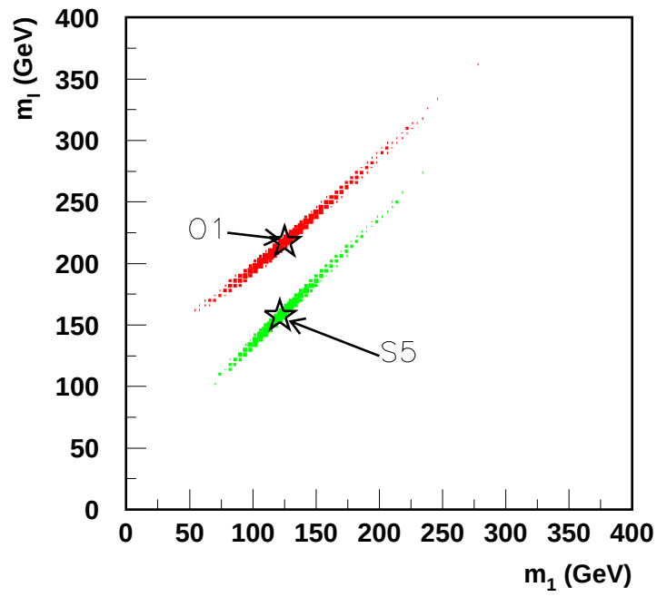
Figure 15: Reconstructed m_l versus m_{\tilde{\chi}_1^0} for O1 and S5 . The stars show the true masses for each model.
