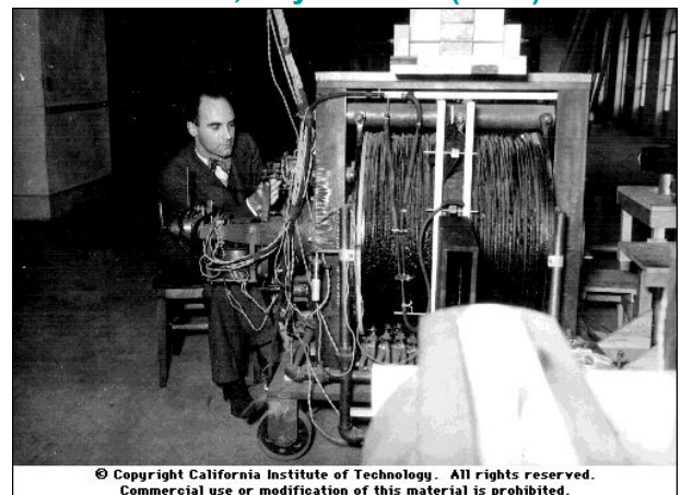
C.D.Anderson, Phys Rev 43 (1933) 491
